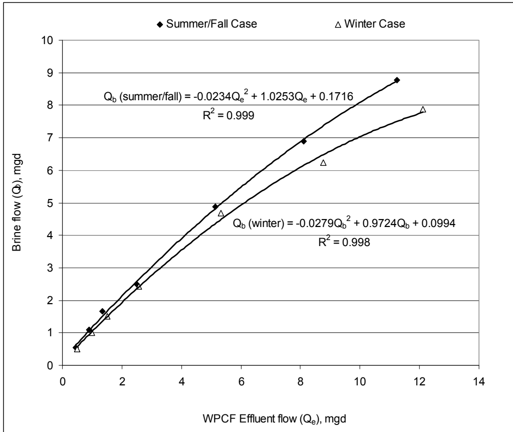
Figure 5-2. Maximum Brine Flow as a Function of Wastewater Effluent Flow to Maintain a Dilution Factor of 139 Line through Points Shows Best-fit Second Order Quadratic
