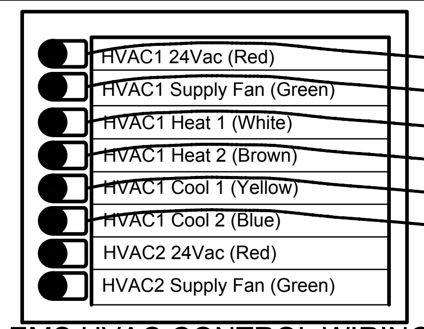
1 EMS-4 EMS HVAC CONTROL WIRING DETAIL N.T.S.
