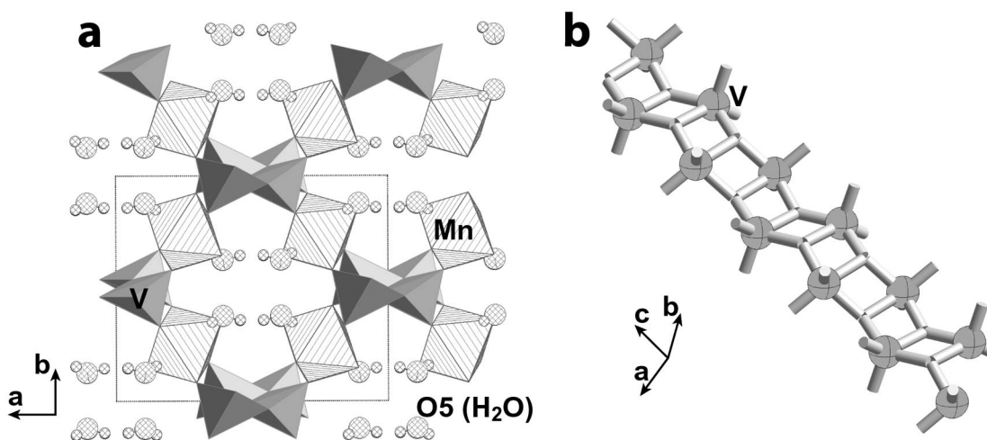
FIG. 2. Crystal structure of ansermetite. (a) Projection of the structure on (001). Gray pyramids are [VO 5 ] groups, and hatched octahedra are [MnO 4 (OH 2 ) 2 ]. The O5-centered H 2 O groups are shown; the O3-centered H 2 O groups belong to the [MnO 4 (OH 2 ) 2 ] octahedron and project on the O5 position on this projection. (b) View of the vanadate chains in ansermetite. The spheres represent V 5+ ions, and the “rods” represent bonds to O 2- ions.
