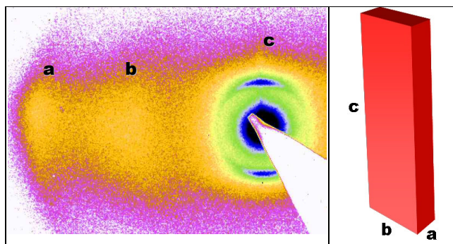
figure 1: biaxial nematic phase.
