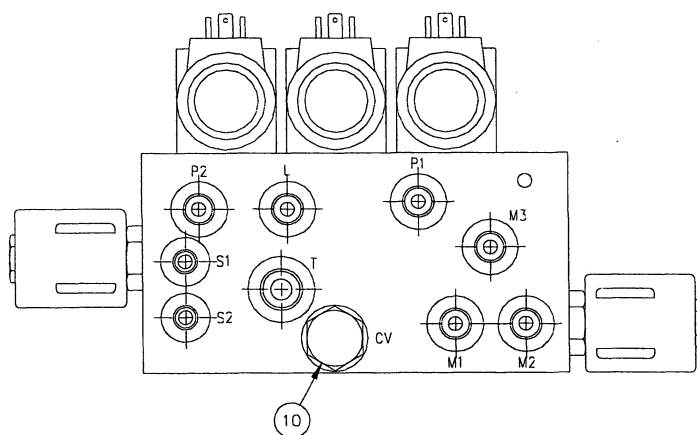
BACK VIEW B-B
