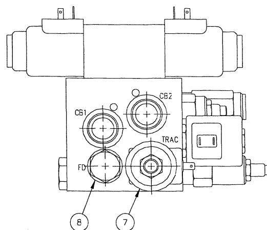
LEFT END VIEW A-A
