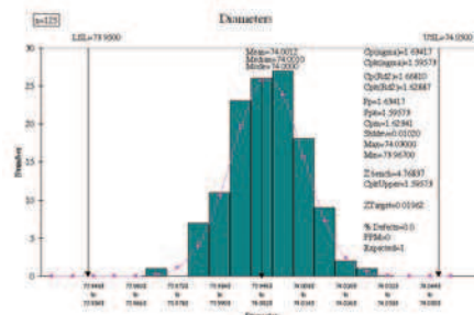
Histograms with Cp Cpk
