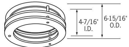
CTR4324V-(CLR, WHT)-P 2AR4(B, F, G, R, Y)
