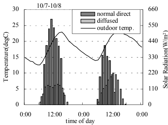
Figure9 Meteorological conditions
