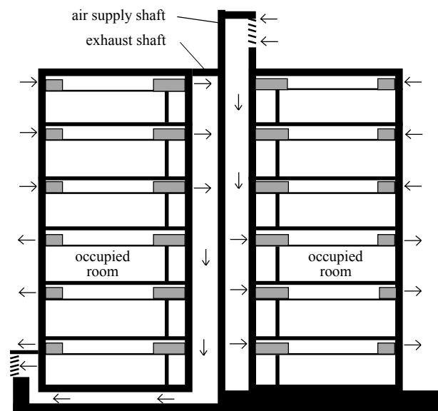
Figure6 Multi-story building section
