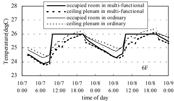
Figure10 Temperature variation
