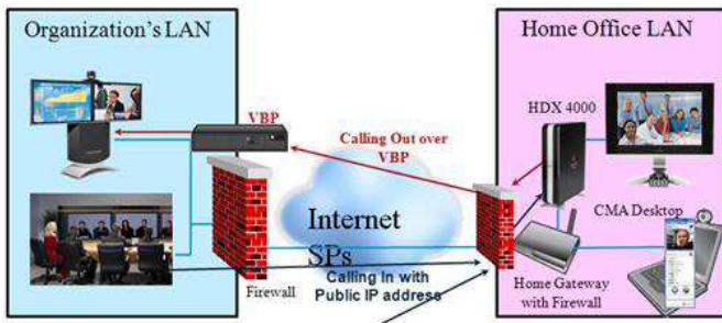
Figure 15. Using VBP at the organization
