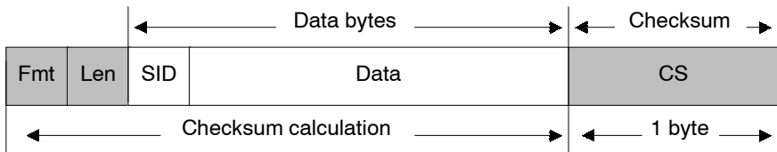
Header without address Information, additional length byte
