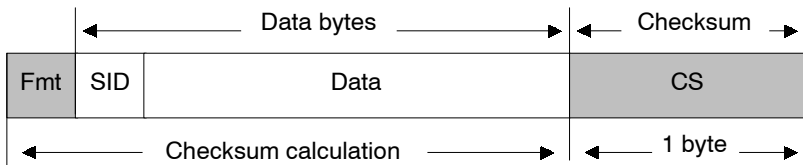
Header without address information, no additional lenght byte
