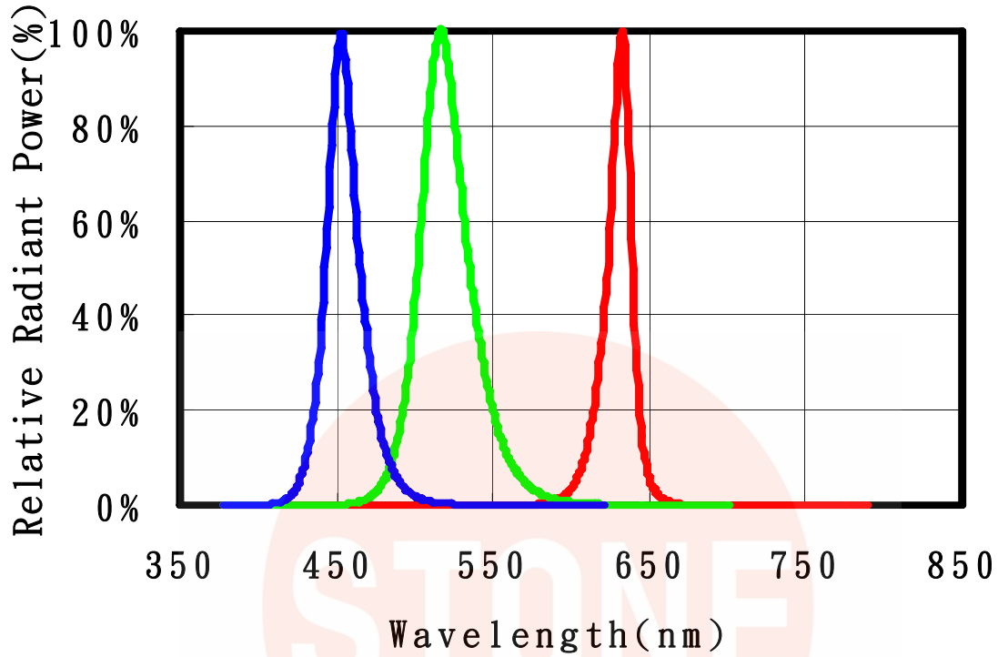
Relative Spectral Power Distribution(Ta=25 )
