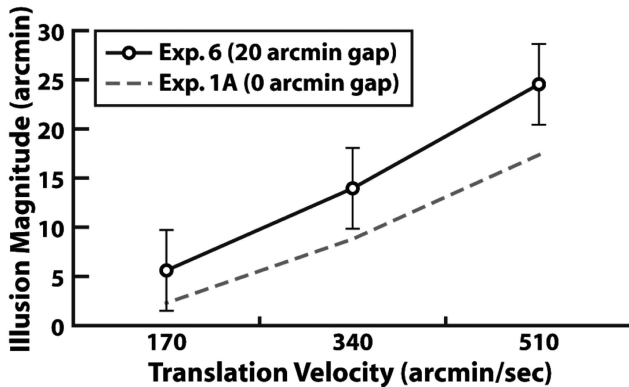
Figure 14. Overall magnitude of the illusion in Experiment 6 (with Experiment 1A data included for reference). Increasing the gap between apertures in the occluding surface caused an increase in the final alignments of the top piece of the rod relative to the bottom piece. Error bars are within-subjects confidence intervals (Loftus & Masson, 1994).
