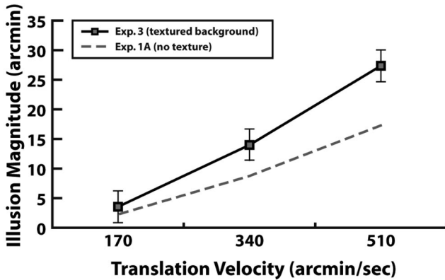
Figure 9. Illusion magnitude as a function of the translation velocity of the rod in Experiment 3. Error bars are within-subjects confidence intervals (Loftus & Masson, 1994).
