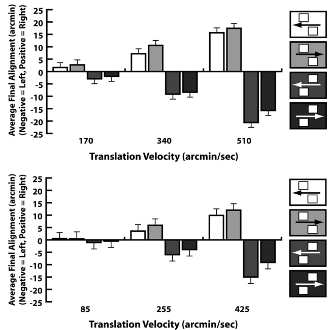
Figure 4. Final adjusted position of top piece of the rod, relative to the bottom piece, by stimulus velocity, motion direction, and aperture configuration for Experiment 1A (top) and 1B (bottom). Participants adjusted the top object fragment to appear aligned with the bottom. Positive alignment values indicate rightward displacement and negative alignment values indicate leftward displacement. Error bars are within-subjects confidence intervals (Loftus & Masson, 1994).
