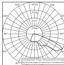
CSA Test Report #: 2586938-6167 XSPA*3HL-U Initial Delivered Lumens: 13,017
