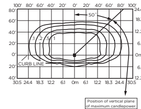
XSPA*HHL-U Mounting Height: 25' (7.6m) A.F.G. Initial Delivered Lumens: 10,942 Initial FC at grade
