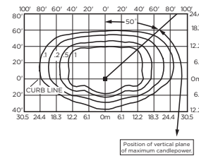
XSPA*3HL-U Mounting Height: 25' (7.6m) A.F.G. Initial Delivered Lumens: 13,418 Initial FC at grade
