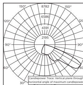
CSA Test Report #: 2586938-6166 XSPA*HHL-U Initial Delivered Lumens: 10,787
