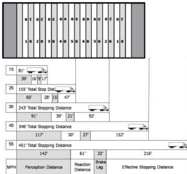
Figure 38: Stopping Distance
