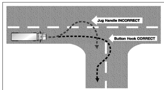
Figure 42: Turning Wide
