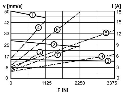
Acme Screw Models Speed and Current vs. Load
