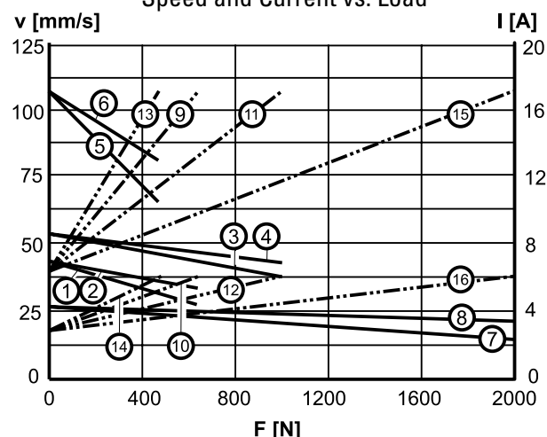
Speed and Current vs. Load
