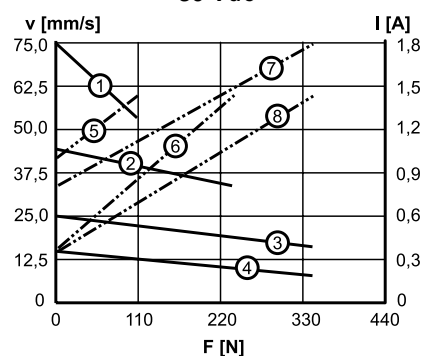
Speed and Current vs. Load
