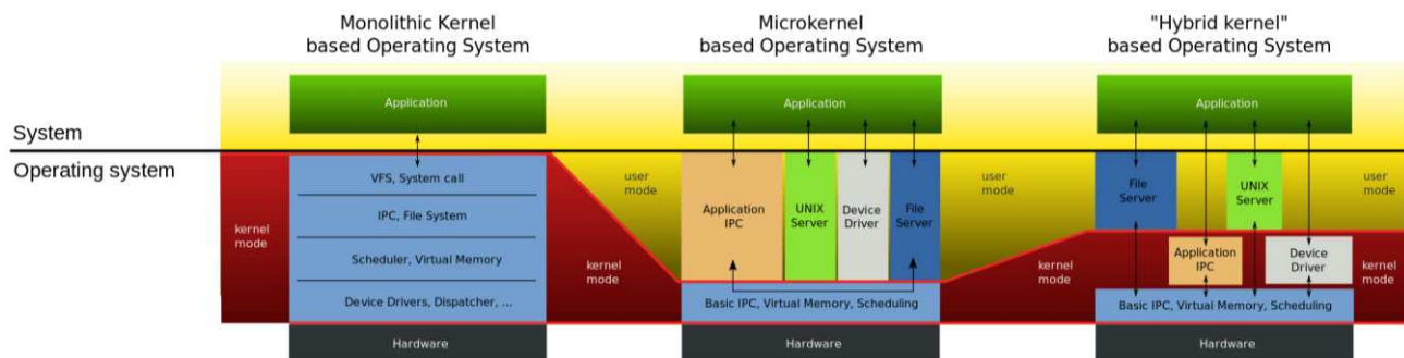
Figure 2: Monolithic & Microkernel structures
