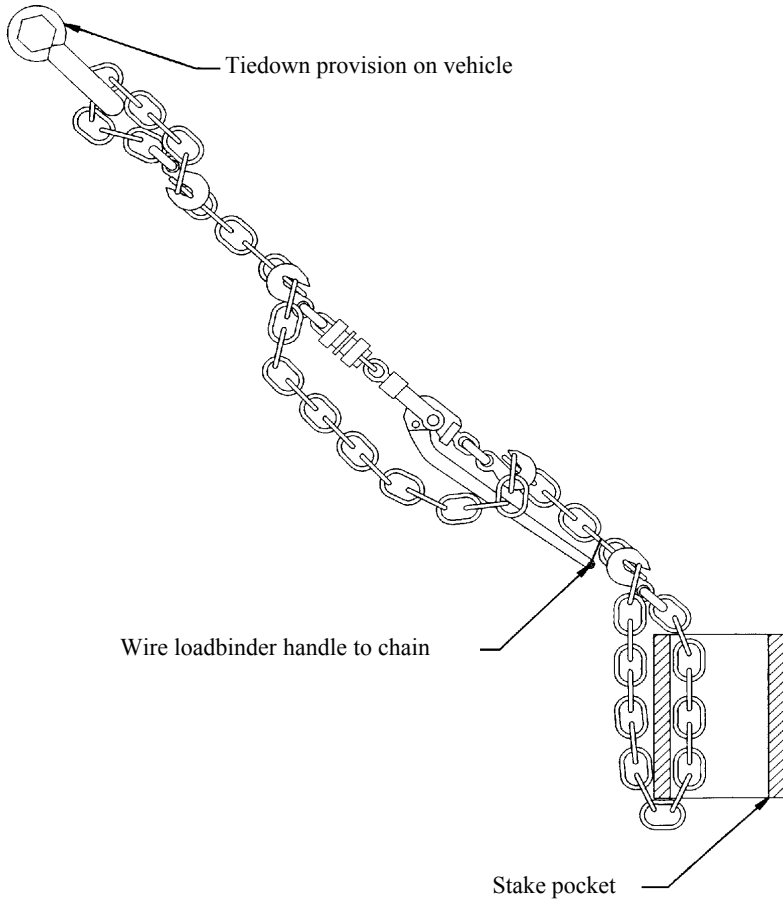
Figure 65. Chain tiedown running through a stake pocket.
