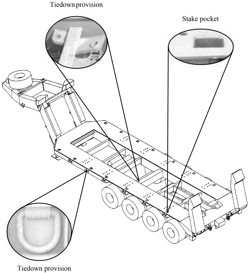
Figure 34. M747 HET.
