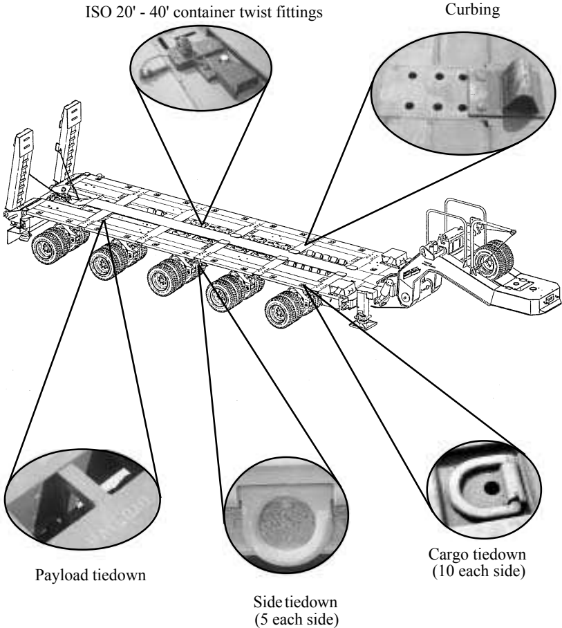
Figure 44. M1000 HET.
