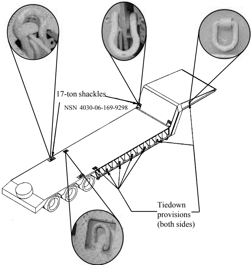
Figure 12. M870A1 semitrailer.
