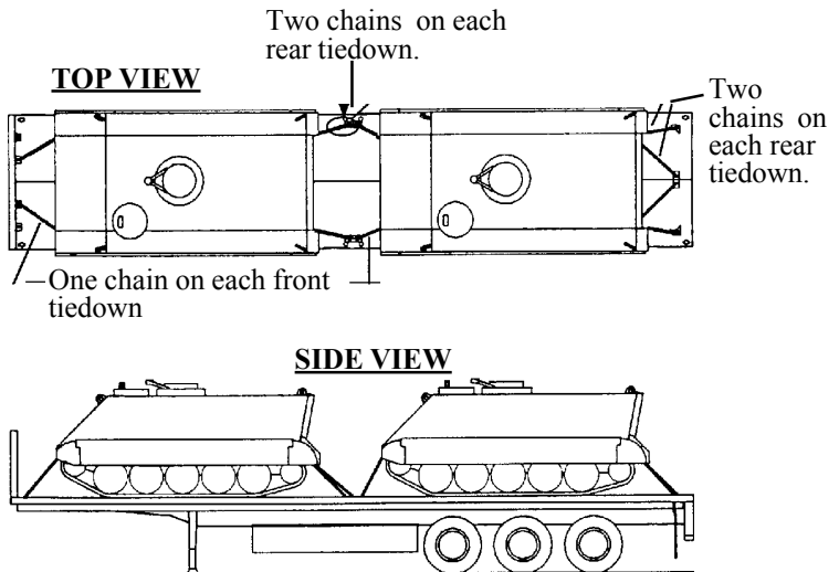
Figure 32. Two M113 variants secured to an M872A3.
