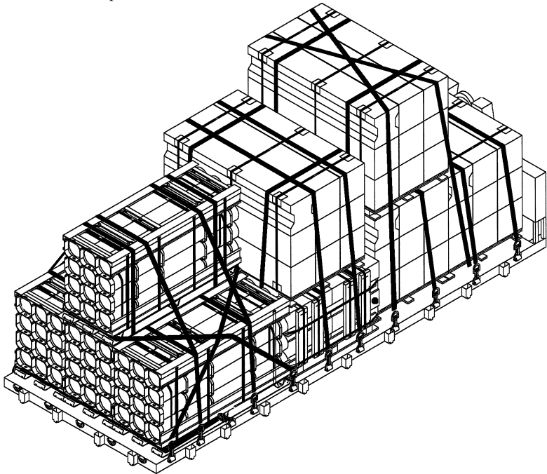
Figure 62. 16-1/2 ton payload on an M1077 A-frame flatrack.
