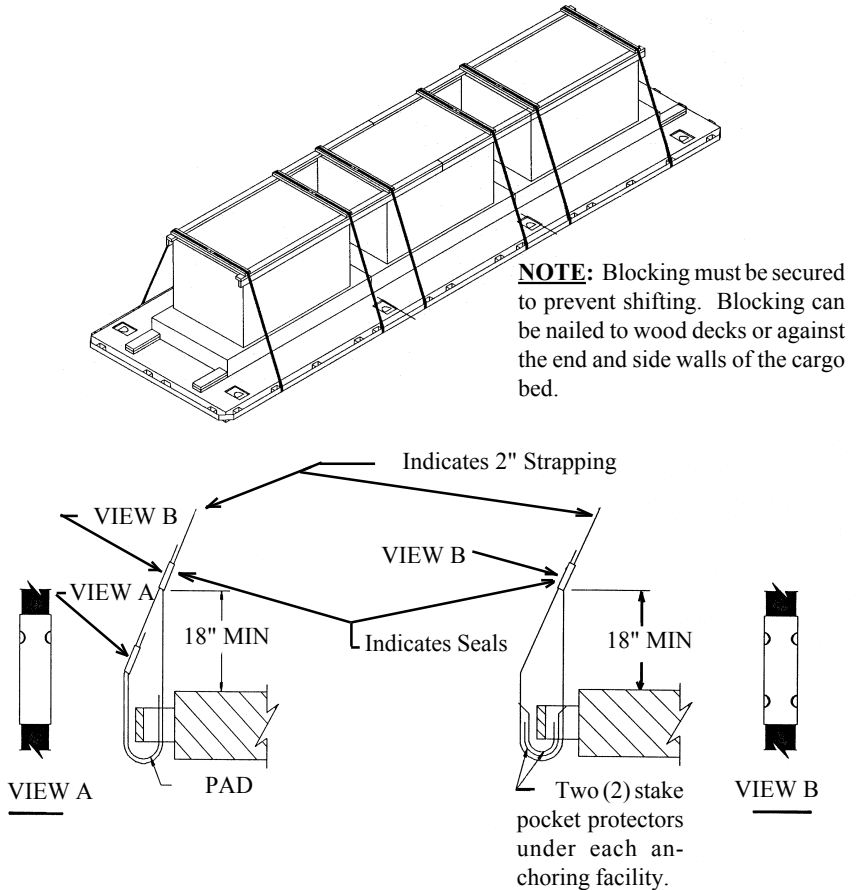
Figure 77. Typical load secured with steel straps and strap anchoring detail.
