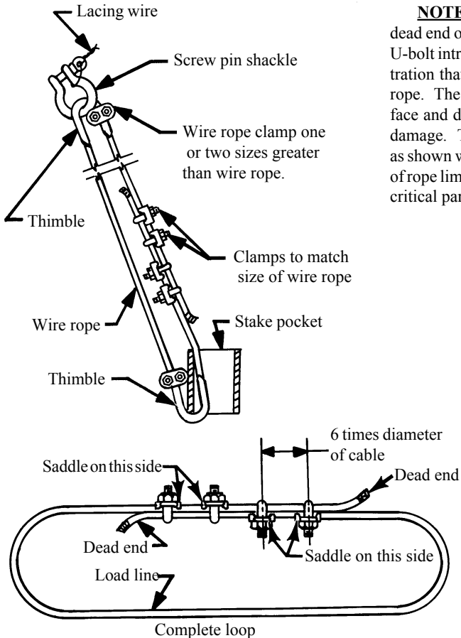
Figure 67. Complete loop wire rope assembly.
