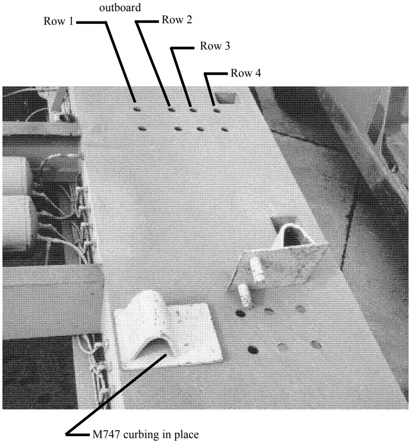
Figure 38. M747 curbing.
