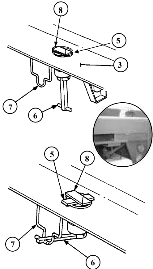
Figure 28. Operation of the M872A3 retractable twist lock.
