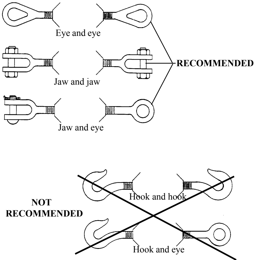
Figure 70. Turnbuckles.
