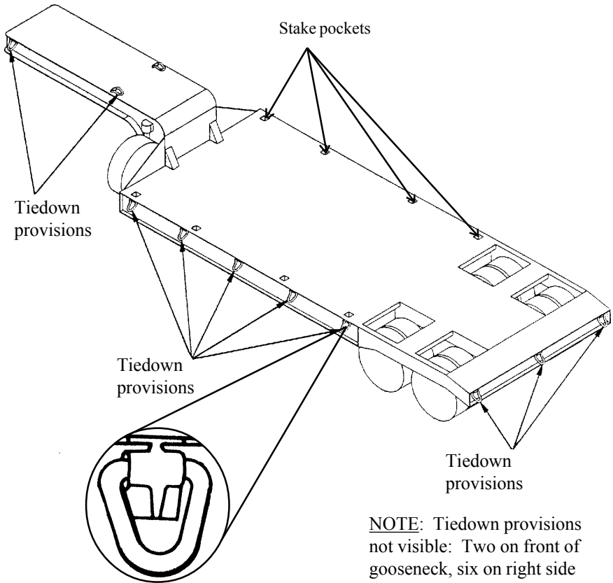
Figure 8. M172A1 semitrailer.
