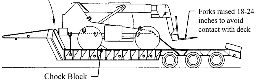
Figure 20. Tiedown configuration of 6K VRRFTL on the M870.
