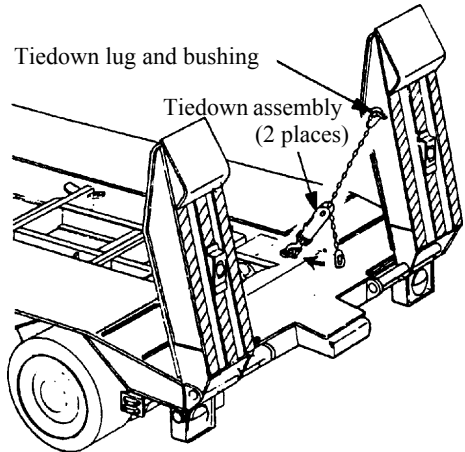
Figure 35. M747 loading ramp tiedown.
