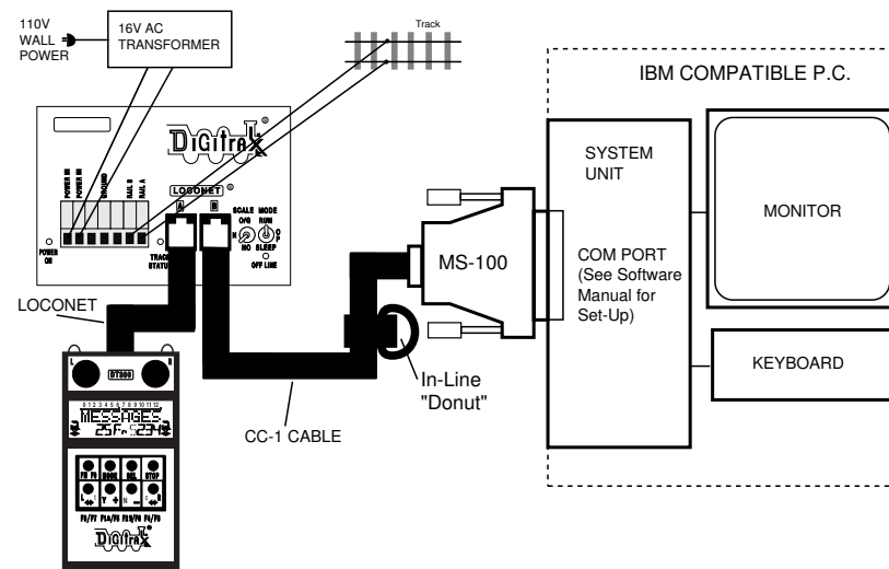
Diagram 1. MS100 Computer Connection Example
