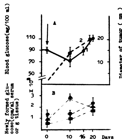
Chart 4. Dynamics of blood glucose and gluconeogenesis in mice with Crocker sarcoma. Designations and conditions as in Chart 1. Glucose- 14 C, derived from 30 \mu Ci, 1.0 ml tyrosine- 14 C, was isolated by paper chromatography. Diameter of the tumor was measured as described (24).
