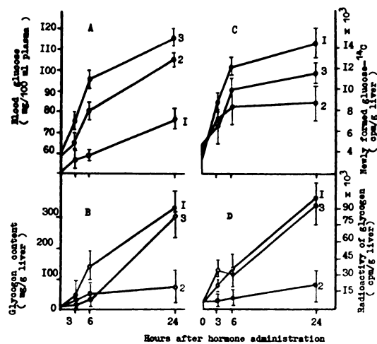
Chart 2. Gluconeogenic response of normal and tumor-bearing mice to cortisol; A , blood glucose levels; B , changes in glycogen content in liver; C , glucose formation from uniformly labeled alanine- 14 C in liver. The radioactive precursor introduced into the animals in succession (2.5 μCi/mouse/day); D , dynamics of glycogen synthesis from glycine- 14 C in liver as revealed by the radioactivity of glycogen. 1, control; 2, mice with Ehrlich carcinoma 8 days after transplantation; 3, mice with Crocker sarcoma 20 days after transplantation. Each point of the curves corresponds to a mean value obtained on 15 ( A ) and 5 ( B , C , D ) animals. Starting from the moment the isotope was introduced, the animals starved for 18 hr (12). At zero time, cortisol, 5 mg/mouse, was given.
