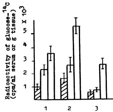
Chart 5. Gluconeogenesis in mice with Guelstein 22a solid hepatoma. Glucose- 14 C was isolated by paper chromatography; 30 μCi tyrosine- 14 C, 1.0 ml/mouse, exposed to the isotope 1 hr. ■, control; □, tumor-bearing animals; 1, blood; 2, liver; 3, kidney. First and 2nd open columns, 10 and 20 days after transplantation, respectively.
