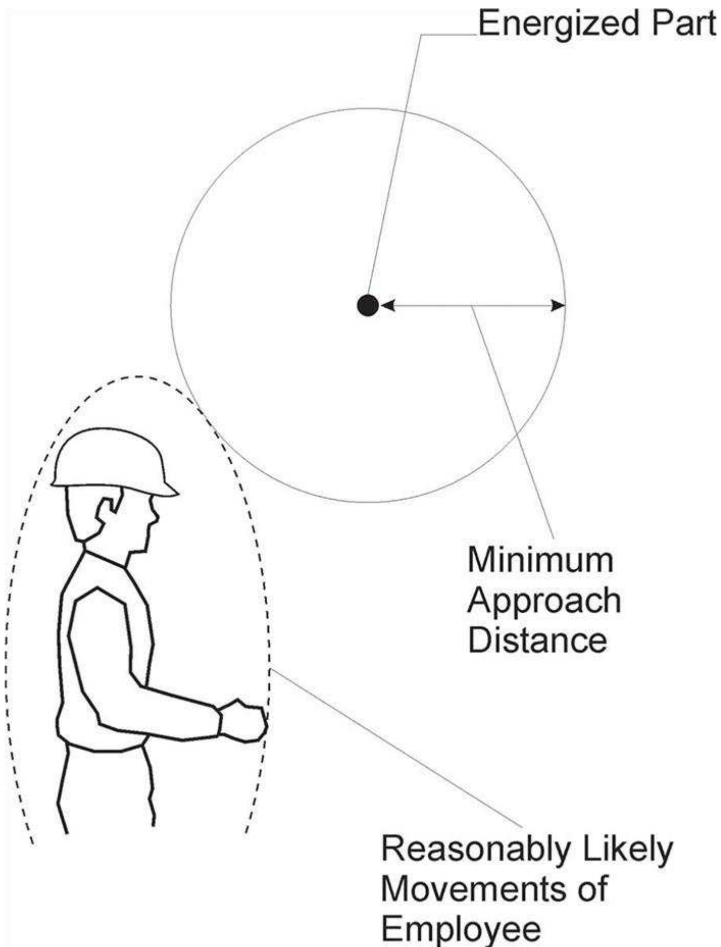
Figure 1 - Maintaining the Minimum Approach Distance
