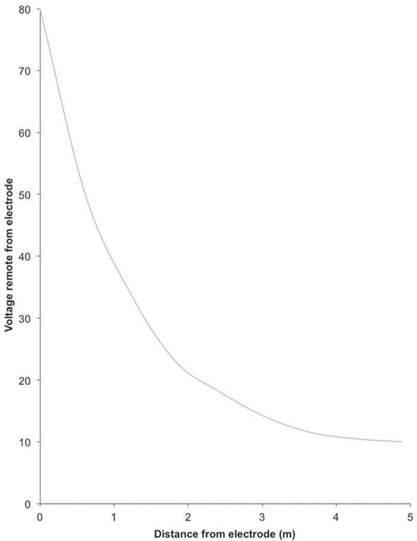
Figure 1 - Typical Voltage - Grandiet Distribution Curve
