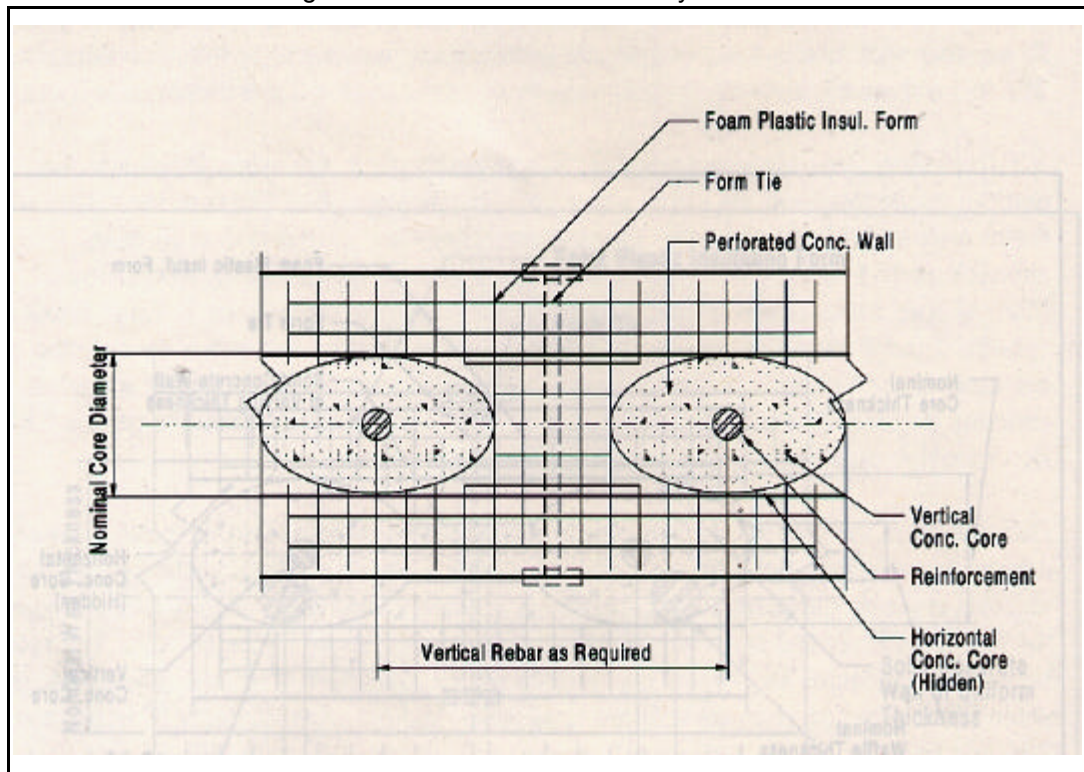
Figure 3: Screen-Grid ICF Wall System
