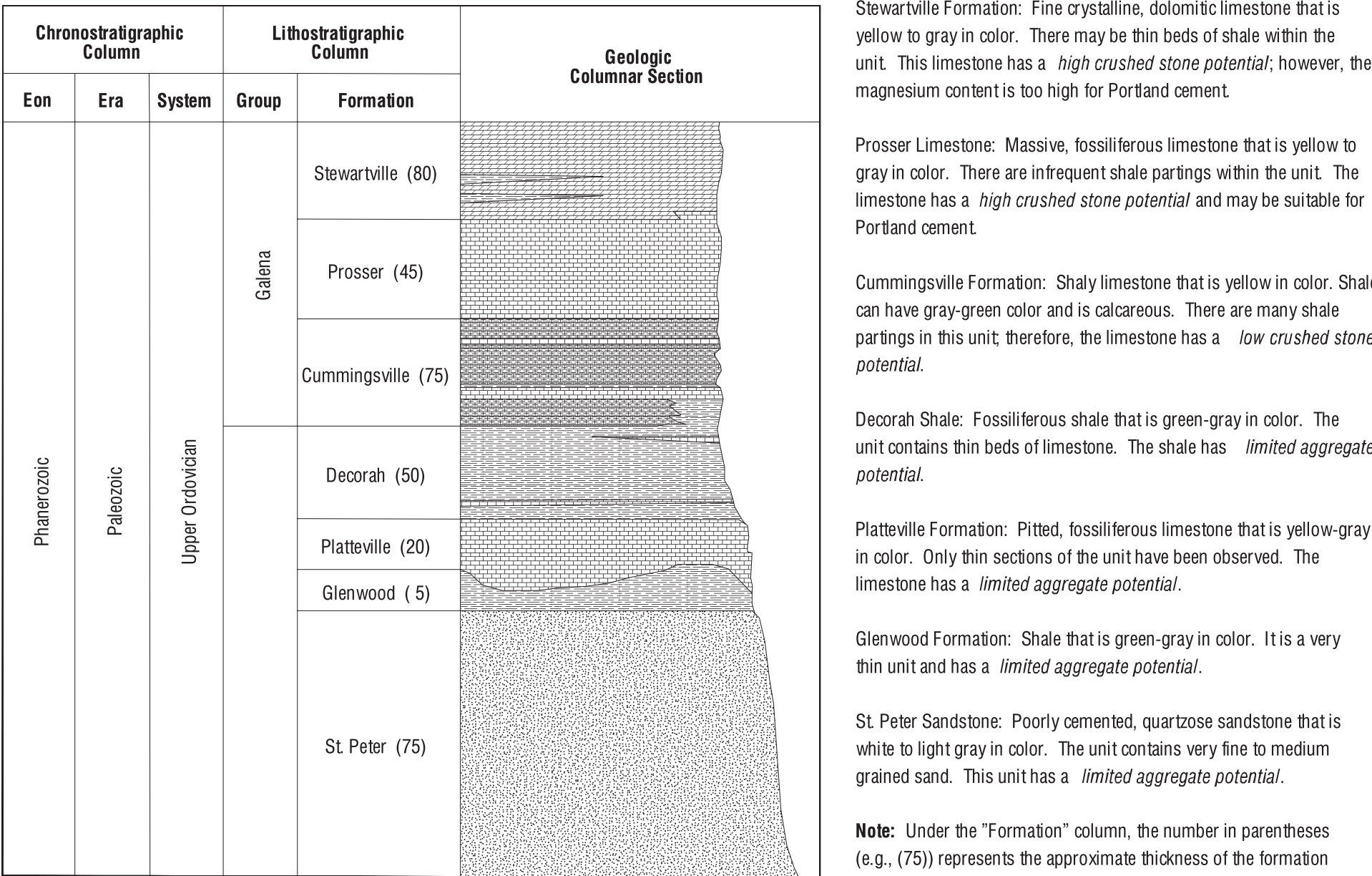
Figure 5. Stratigraphic column of bedrock units exposed in Dodge County (Adapted from Mossler, 1987, and Minnesota Geological Survey, 2001)
