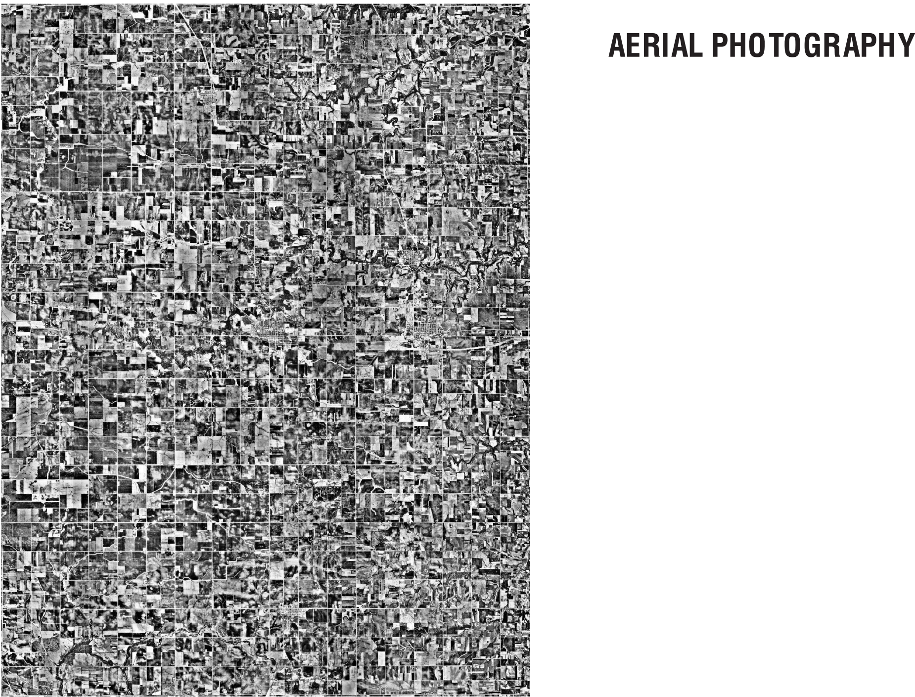
Figure 2. This aerial photography mosaic is composed of Digital Orthophotoquads (DOQs), that is, computer-readable images of aerial photography, that are available from the U.S. Geological Survey (USGS). The aerial photographs were taken in April 1991 and April 1992, from an airplane that was at 20,000' above the land surface using film that was 10" wide. The photographs were then scanned at a 1-meter resolution to create the 1:12,000 quarter-quad DOQ products. For this mosaic, the scanned photographs were resampled at a 10-meter resolution and combined into a county-wide image.
