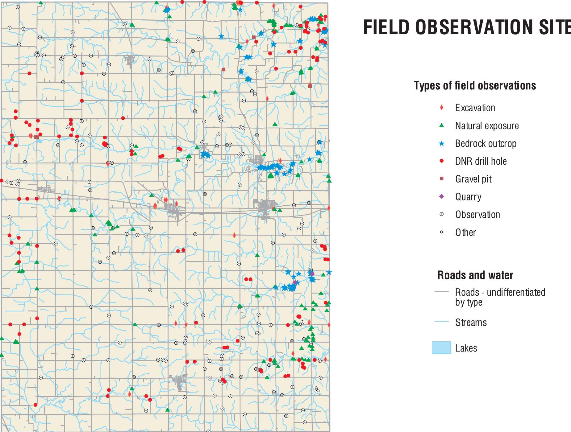
Figure 4. Field work was completed during the summer and fall (July to November) of 2001. Field observation sites consisted of bedrock outcrops, natural exposures, excavations, 8" diameter auger drill holes, gravel pits, and quarries. Every accessible road in the county was traveled looking for these sites to help determine the landform expressions. Field observations were recorded at approximately 420 sites throughout the county.
