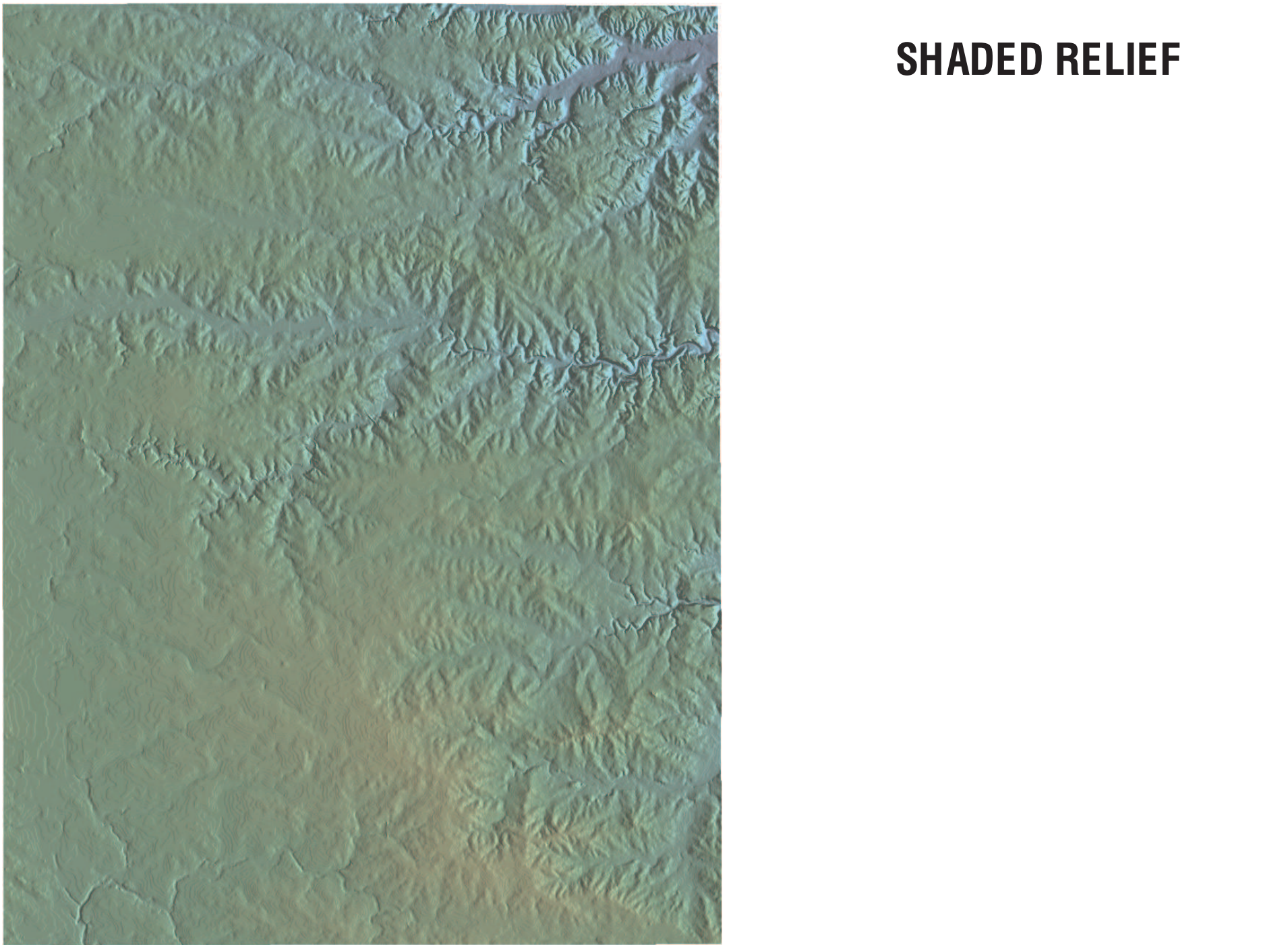
Figure 3. The shaded relief plot of Dodge County was derived from Digital Elevation Model data and the use of a hillshading command to make the elevations appear 3-dimensional by adding bright spots and shadows as they might be cast by the sun. Digital Elevation Models (DEMs) are digital files storing terrain elevation at regularly spaced, horizontal intervals derived from U.S. Geological Survey (USGS) 7.5-minute quadrangles. The DEM data used in this case are available at 30-meter spacing from the USGS.
