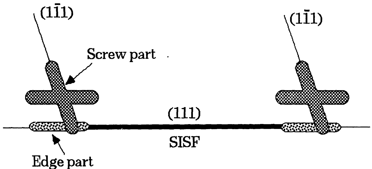
Fig. 8. The schematic picture of the cores of the superpartials forming the dislocation dissociated according to the reaction 1/2[1\bar{1}0] = 1/3[1\bar{1}2] + 1/3[2\bar{1}\bar{1}] .
