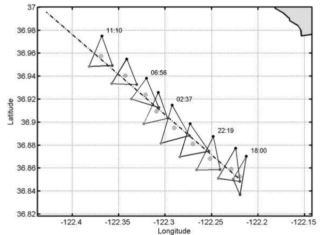
Figure 1. Paths of three underwater gliders and their center of mass over a 16-hour sea trial in Monterey Bay, August 6, 2003. From E. Fiorelli et al., "Multi-AUV Control and Adaptive Sampling in Monterey Bay," 2004.
