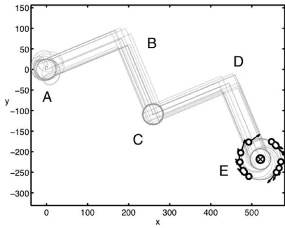
Figure 4. Twelve point particles starting in random positions near (0,0) first congregate in a circle, then head off in an east-northeast direction (A), shift to the southeast (B), pause in a circular formation before repeating the zigzag (C and D), and end by enlarging the circle (E). From Rodolphe Sepulchre, Derek Paley, and Naomi Ehrich Leonard, "Stabilization of Planar Collective Motion, Part I: All-to-All Communication," 2005.
