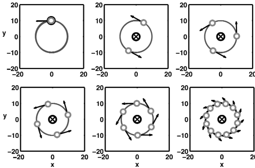
Figure 3. Six simulations of 12 particles, each corresponding to a different symmetric pattern for the particles moving around a circle. Figure courtesy of Naomi Ehrich Leonard.
