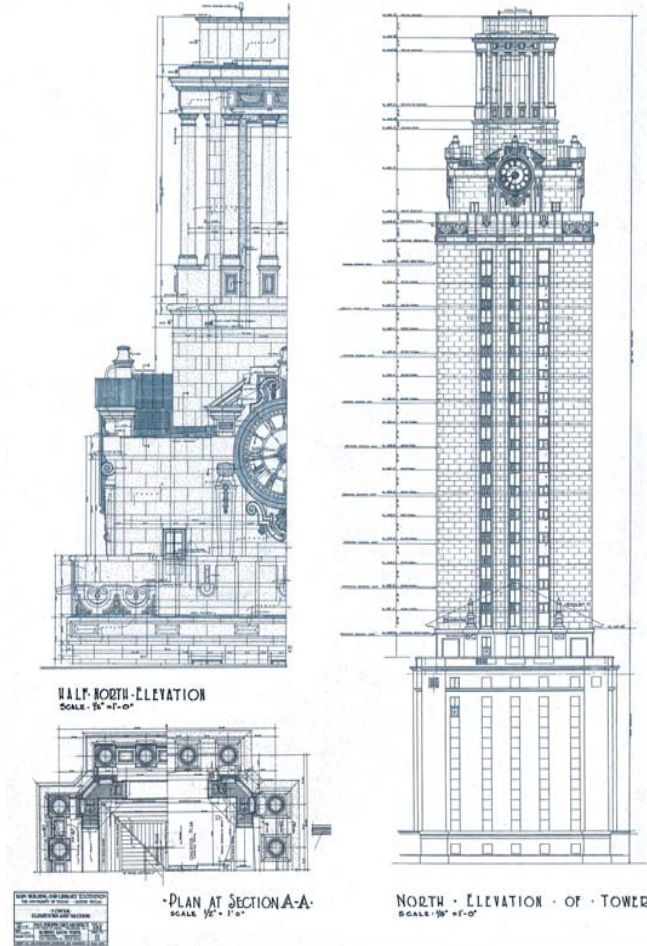
UT Tower Construction Drawing
