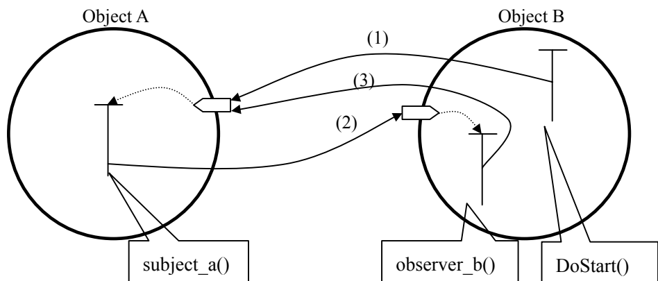
Fig 1-4 Example of an inter-object communication
