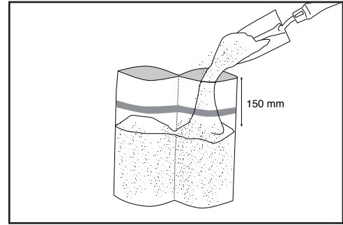
Figure 22-A: Filling the sandbag
