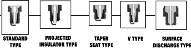
CROSSCUTS & GAP STYLES OF SPARK PLUGS
