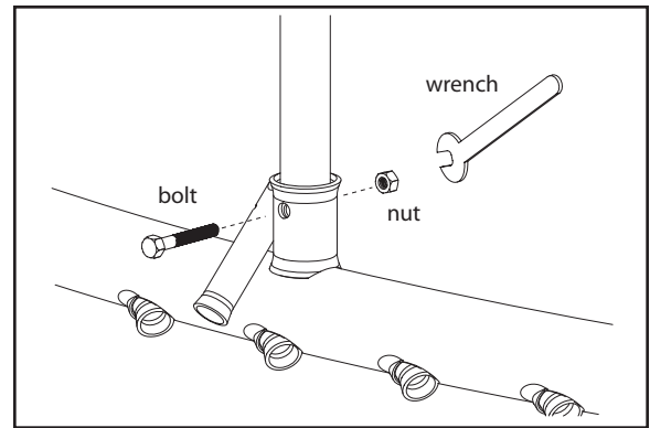
Figure 5: Fastening the legs to the frame
