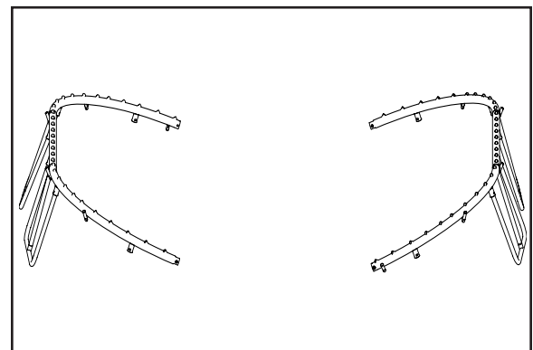
Figure 6-A: Turning the two U shaped sections over
