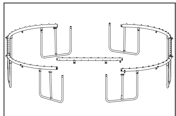
Figure 6-B: Adjusting spacing for straight section
