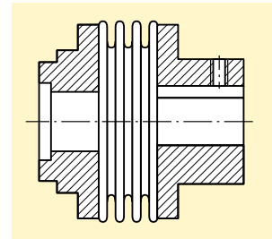
Series AKN/XX Version with special hub on both sides
