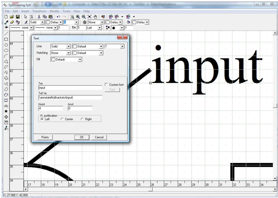
Figure 21: Annotation Alignment
