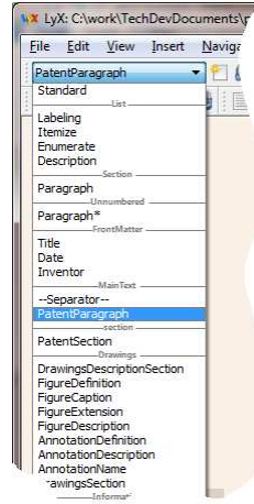
Figure 3: LyX Environments
