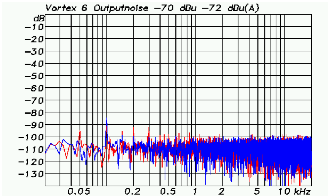
Fig. 6: Interference spectrum at output (CH1,CH2)
