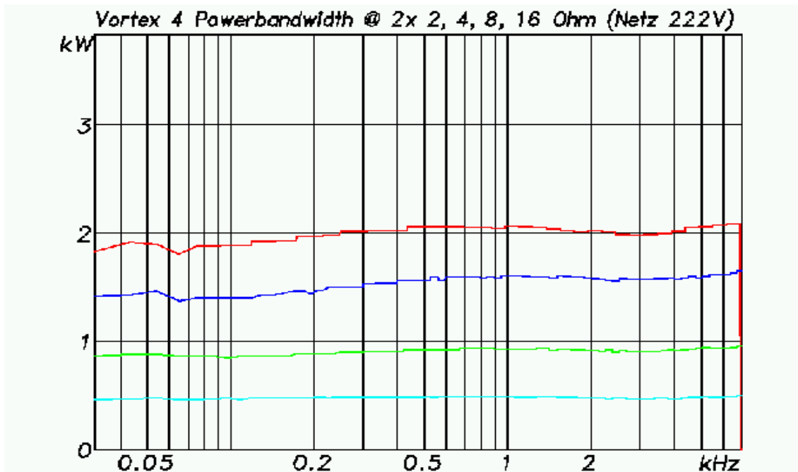
Fig. 13: Two-channel cont. power at 1% THD into 2(red), 4(blue), 8(green) and 16(light blue) ohms
