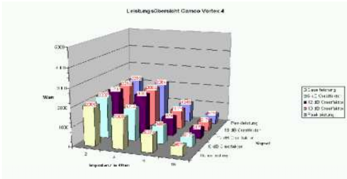
Fig. 15: Performance diagram for one channel with simultaneous load applied to all channels
