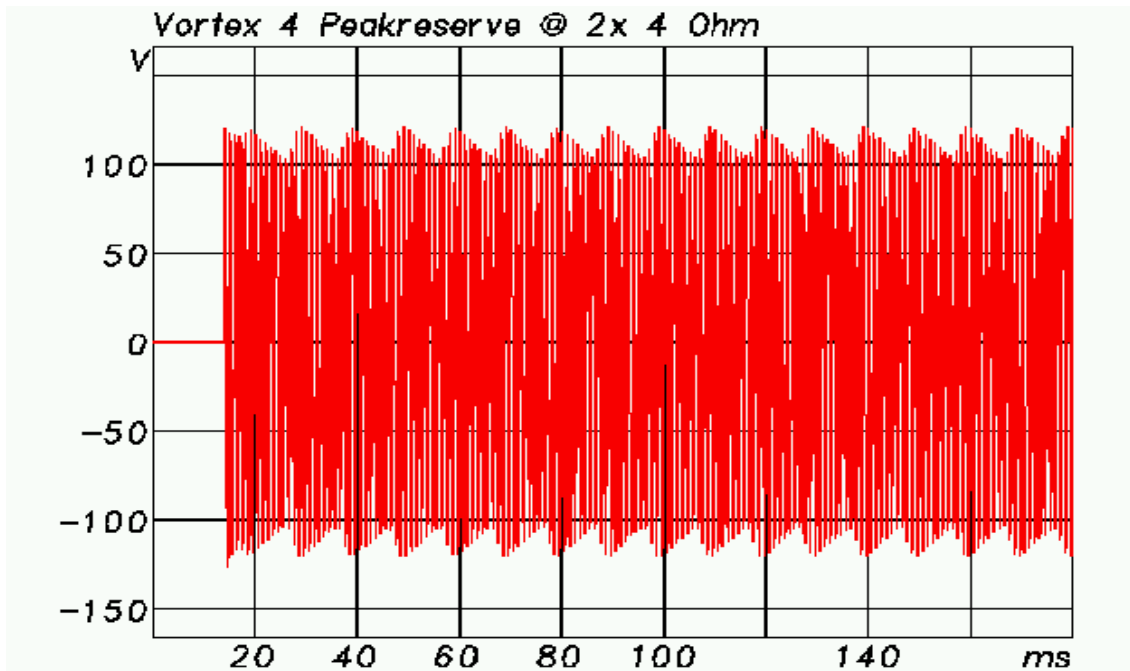
Fig. 14: Peak reserves, 2-channel, into 4-ohm load
