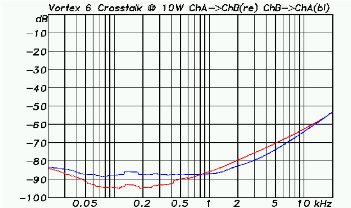
Fig. 3: Crosstalk attenuation (CH1->CH2,CH2->CH1)
