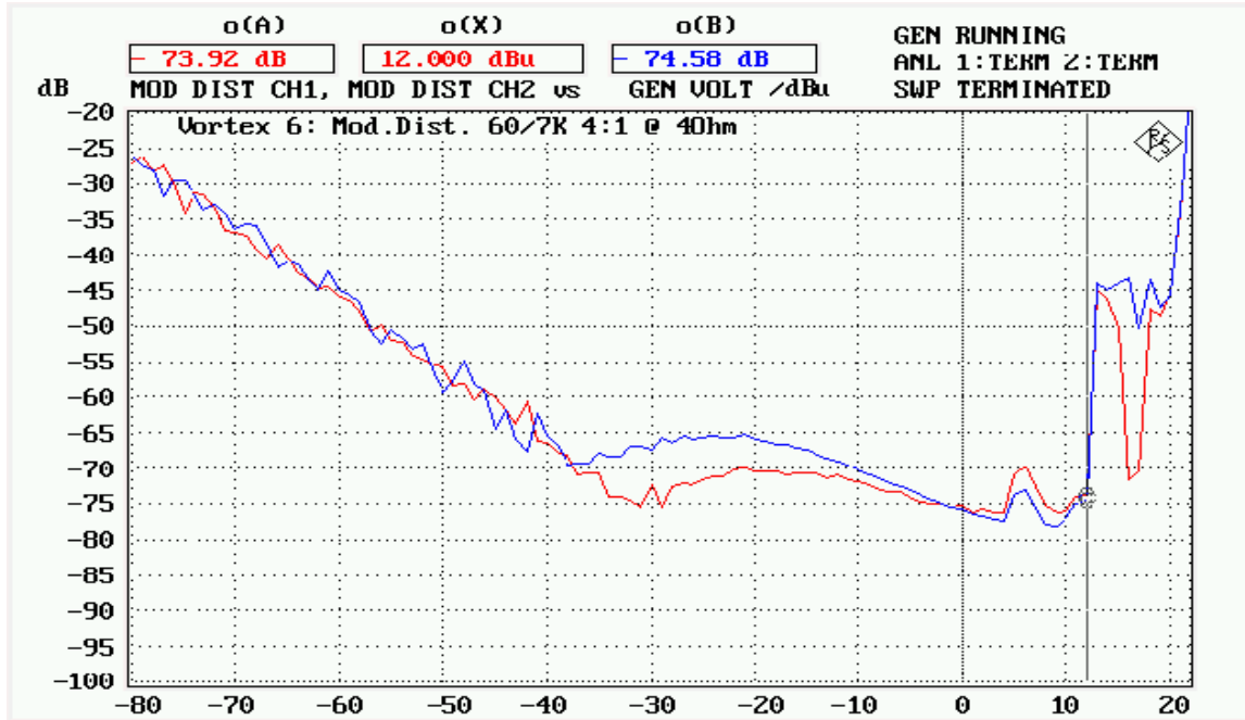
Fig. 11: Modulation distortion according to SMPTE (60 Hz and 7 kHz) into 2x4-ohm load (CH1,CH2)
