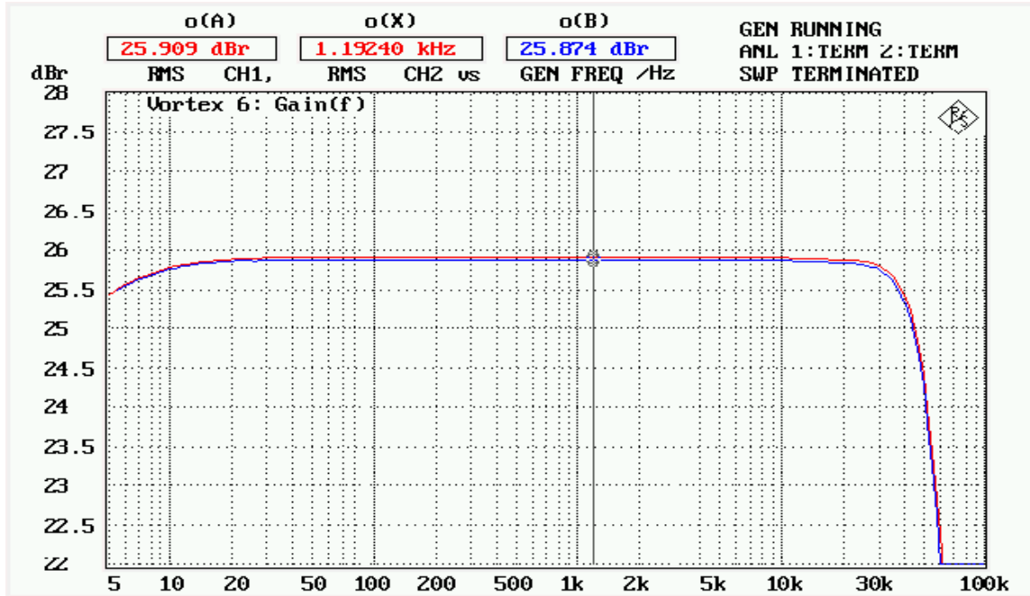
Fig. 1: Gain vs. frequency (CH1,CH2)
