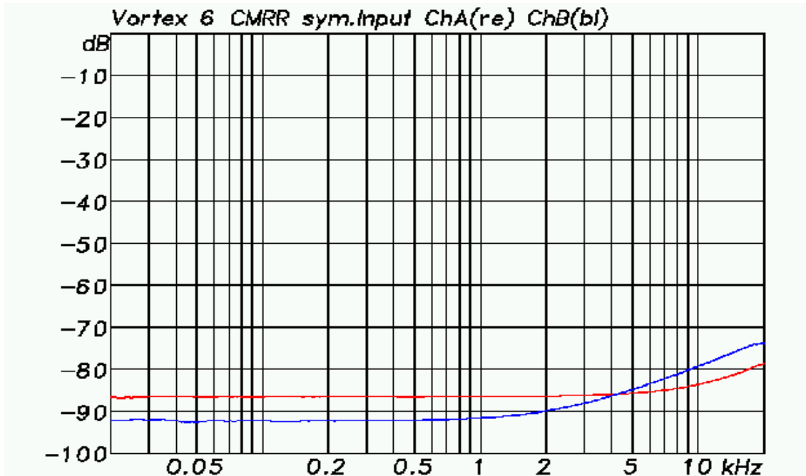
Fig. 5: Common mode rejection (CH1,CH2)
