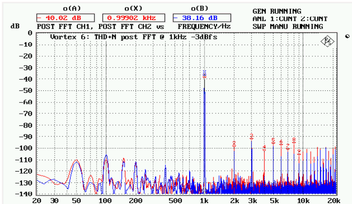
Fig. 8: Distortion spectrum at 1 kHz and into 2x4-ohm load (CH1,CH2), 3 dB under full load (basic oscillation at 1 kHz attenuated by 40 dB)
