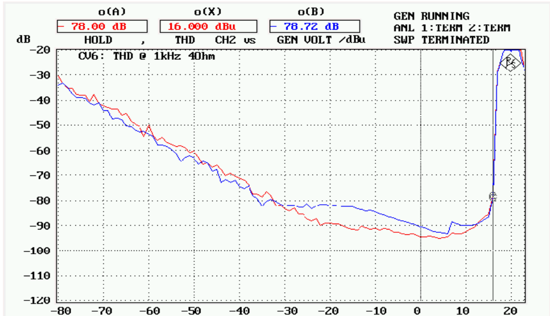
Fig. 7: Total harmonic distortion (THD) at 1 kHz and into 2x4-ohm load (CH1,CH2)
