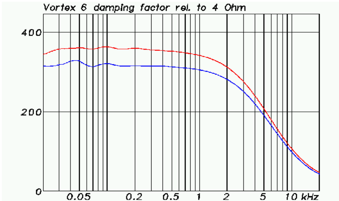
Fig. 4: Damping factor into 4-ohm load vs. frequency (CH1,CH2)
