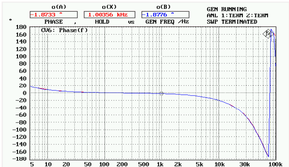
Fig. 2: Phase response vs. frequency (CH1,CH2)
