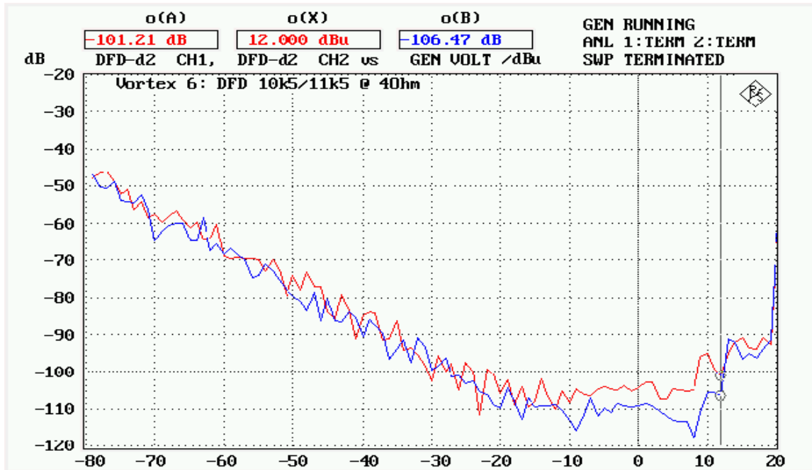
Fig. 12: Difference tone distortion (10.5 kHz and 11.5 kHz) into 2x4-ohm load (CH1,CH2)
