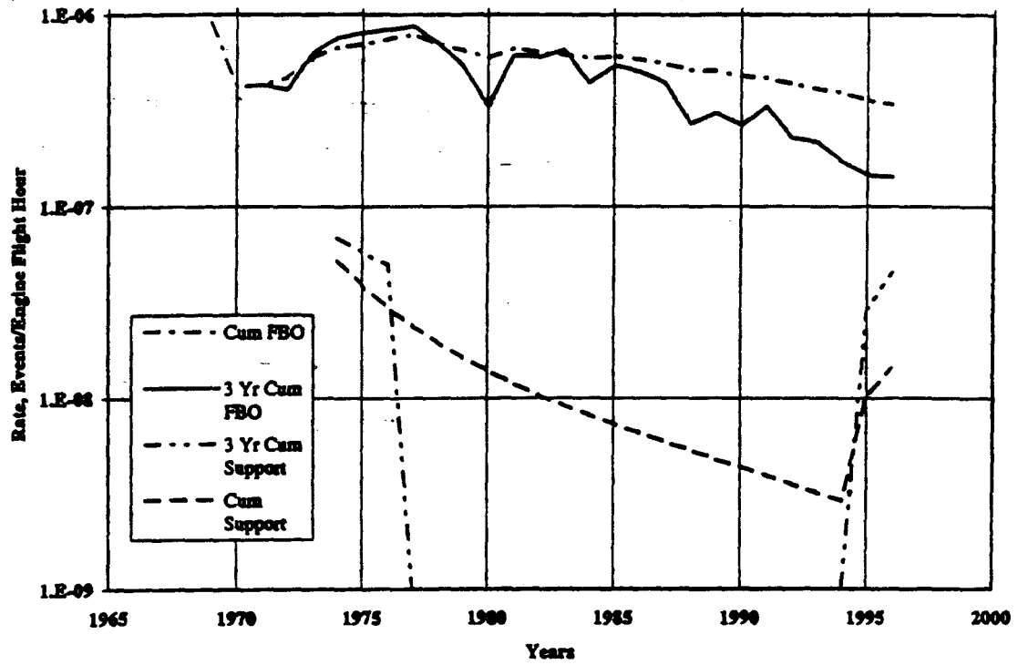
Figure 3.7 Fan Rotor Blade and Support Loss Rate Trends
