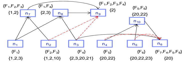
(e) Removing redundant links from UNL.
