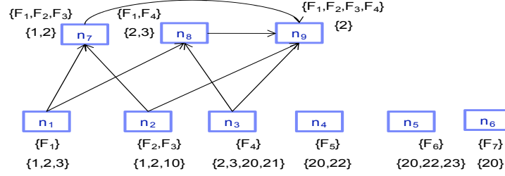
(c) Merging new nodes on n_9 using rule R_2 .
