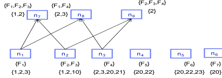
(b) Generating nodes n_7 , n_8 , and n_9 using rule R_1 .
