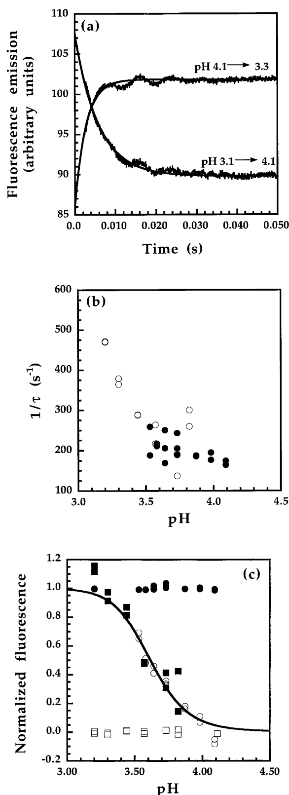
Figure 2. Kinetics of the pH-induced I_a \rightleftharpoons I_b interconversion. The starting pH is either 3.1 or 4.1. Representative time traces for jumps from pH 3.1 to pH 4.1 and from pH 4.1 to pH 3.3 are shown. Conditions: 2 mM Na citrate/citric acid, 30 mM NaCl, 4.5°C, final protein concentration is 10 \mu M after 1:1 dilution. (a) Kinetic traces fitted to a single exponential equation. At higher initial concentrations, a small fluorescence decrease occurs
