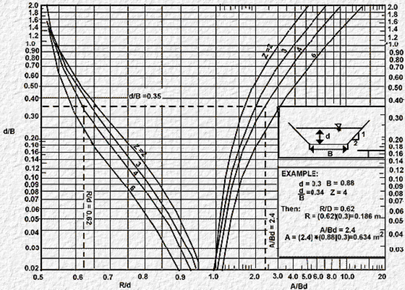
Chart 4. Geometric Design Chart for Trapezoidal Channels
