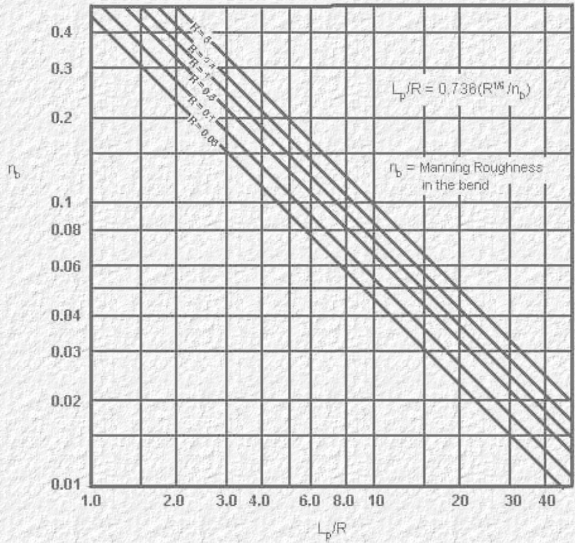
Chart 11. Protection Length, L_p , Downstream of Channel Bend
