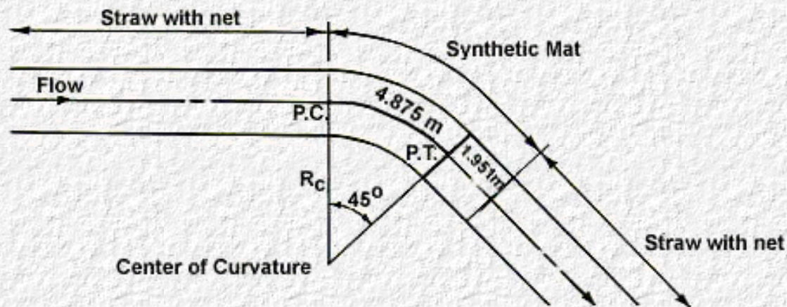
Figure 20. Location Sketch of Flexible Linings for Example 5
