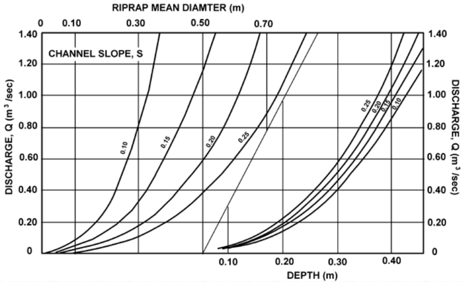
Chart 15. Steep Slope Riprap Design, Triangular Channel z=3
