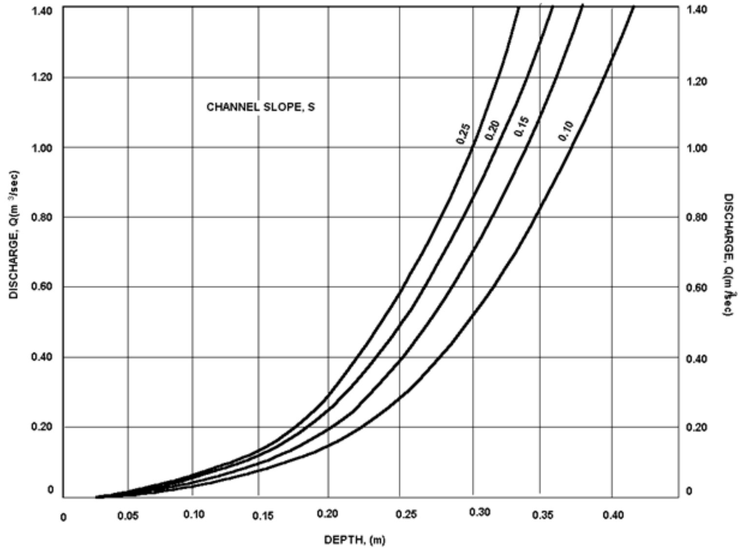
Chart 19. Steep Slope Gabion Mattress, Triangular Channel, Z=3
