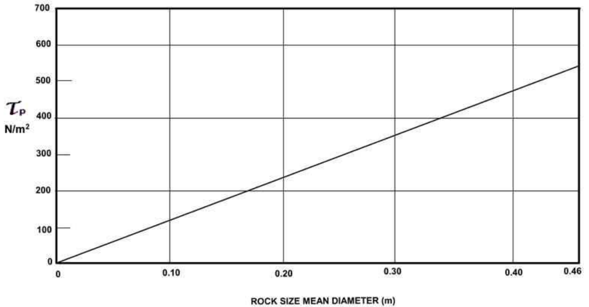
Chart 23. Permissible Shear Stress for Gabion Mattress versus Rock Fill Size
