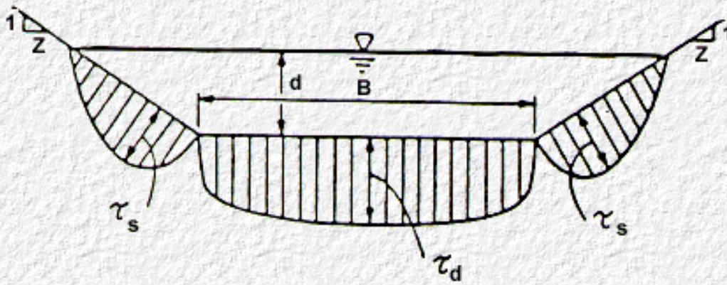
Figure 18. Typical Distribution of Shear Stress
