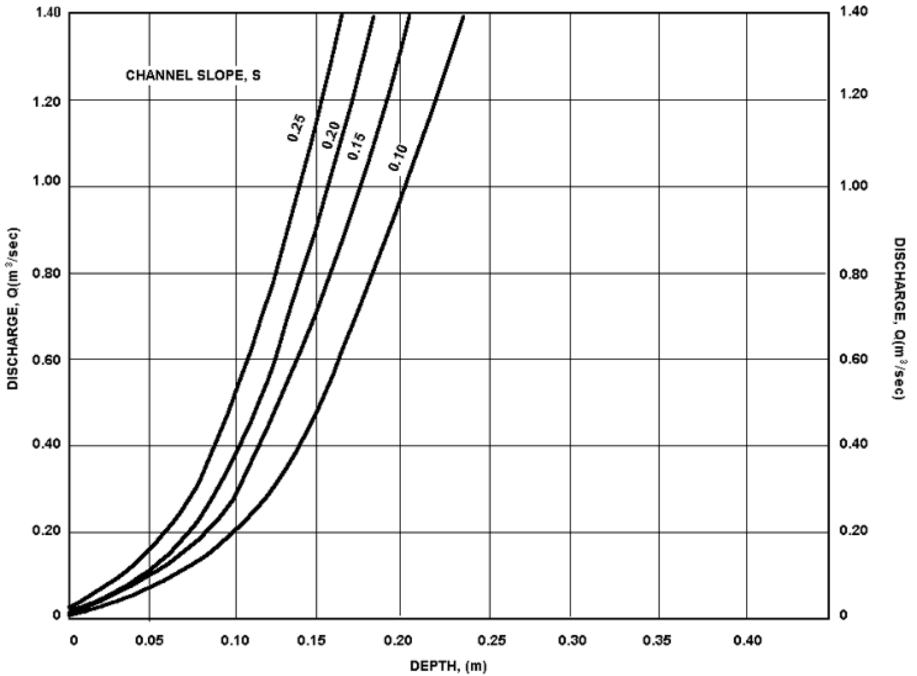
Chart 22. Steep Slope Gabion Mattress, B=1.8m, Z=3
