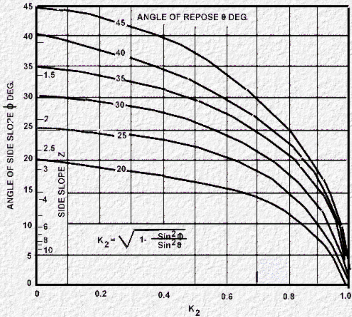
Chart 14. Tractive Force Ratio, K_2 (8)
