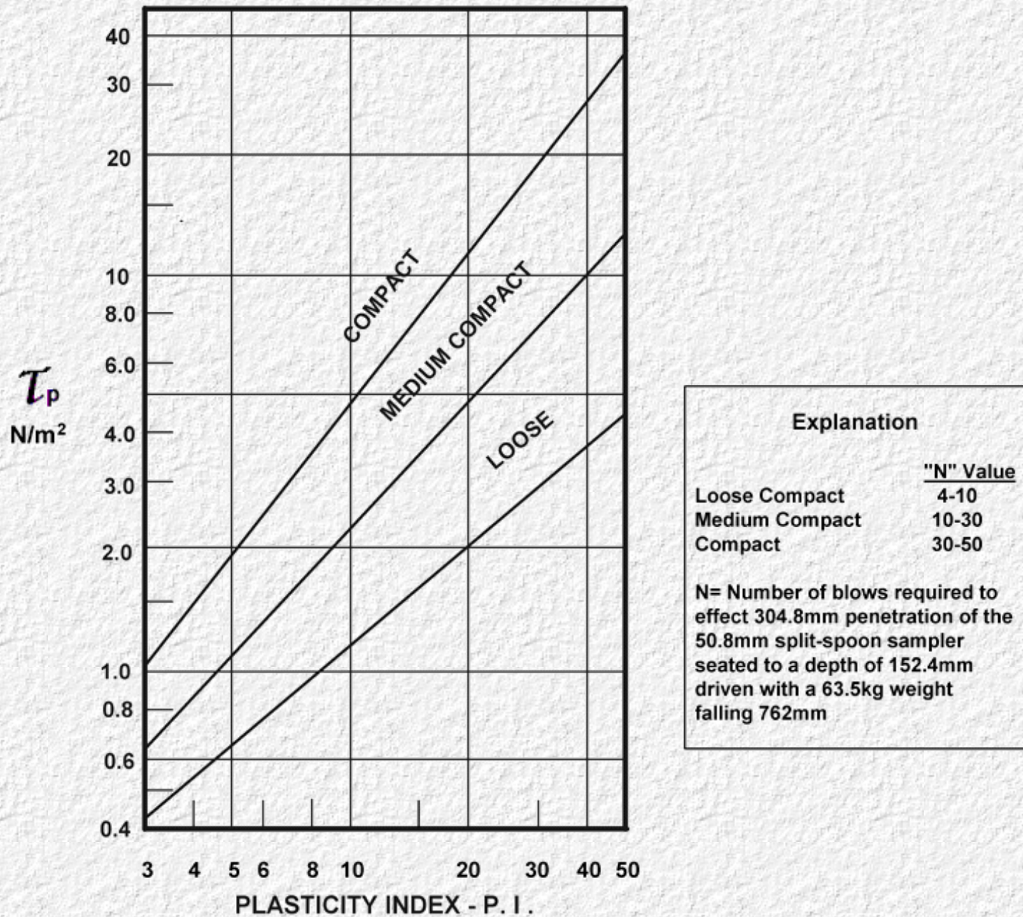
Chart 2. Permissible Shear Stress for Cohesive Soils (after 16)
