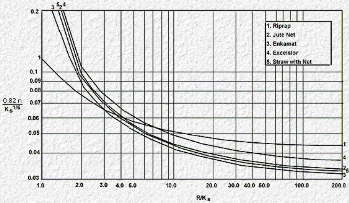
Figure 30. Manning's n versus Relative Roughness for Selected Lining Types.
