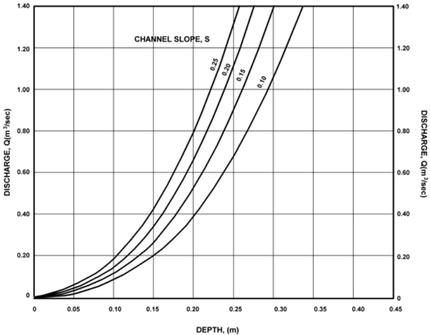
Chart 20. Steep Slope Gabion Mattress, B=0.6m, Z=3
