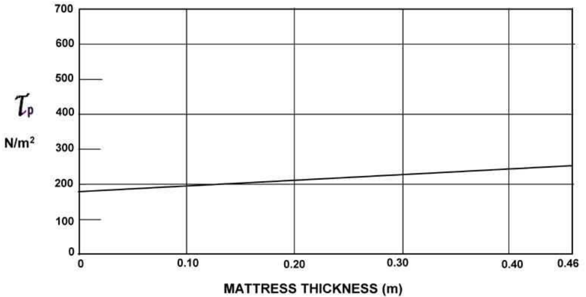
Chart 24. Permissible Shear Stress for Gabion Mattress versus Mattress Thickness
