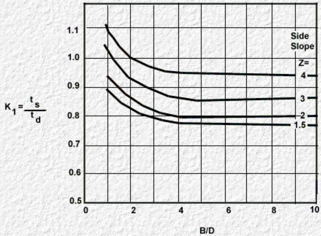
Chart 13. Channel Side Shear Stress to Bottom Shear Stress Ratio, K_1 (8)
