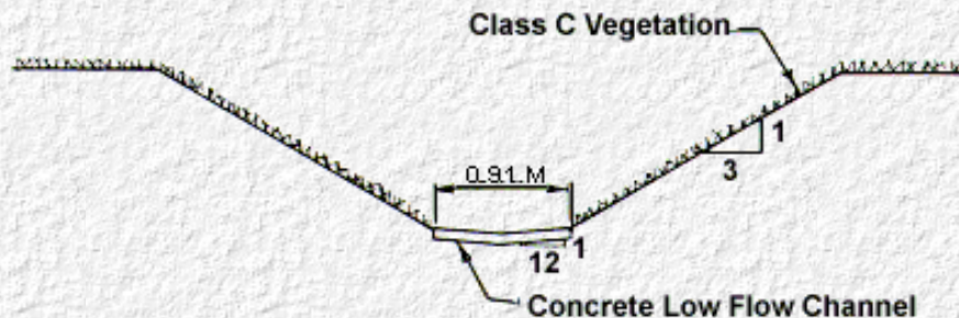
Figure 26. Compound Lining Example
