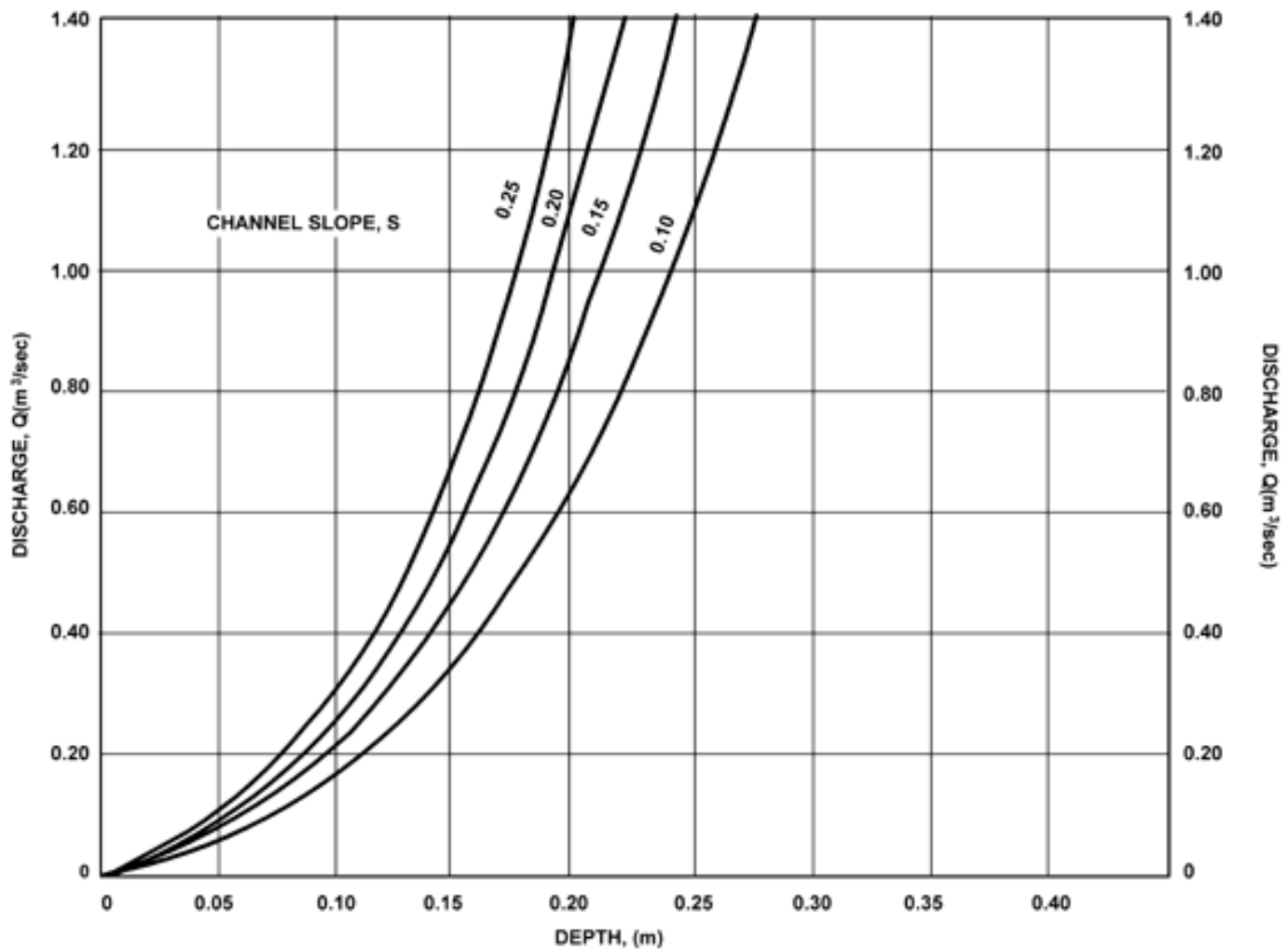
Chart 21. Steep Slope Gabion Mattress, B=1.2m, Z=3
