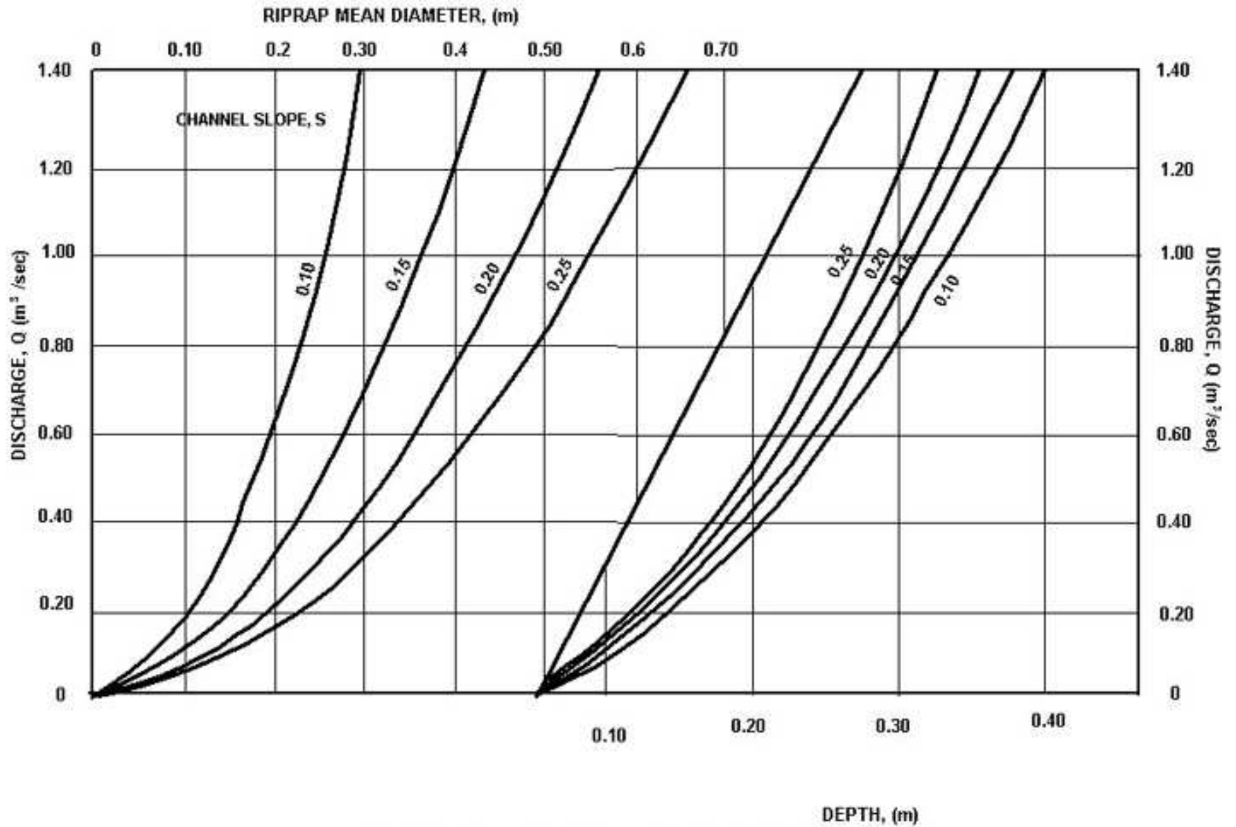
Chart 16. Steep Slope Riprap Design, B=0.6m, Z=3
