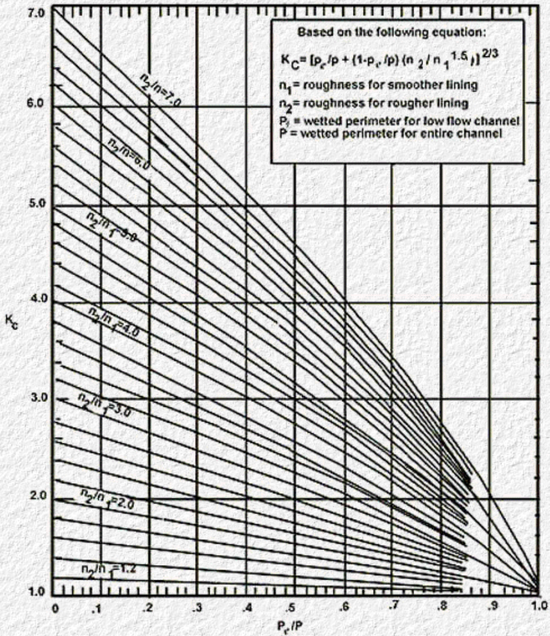
Chart 25. Roughness Factor for Compound Channel Lining
