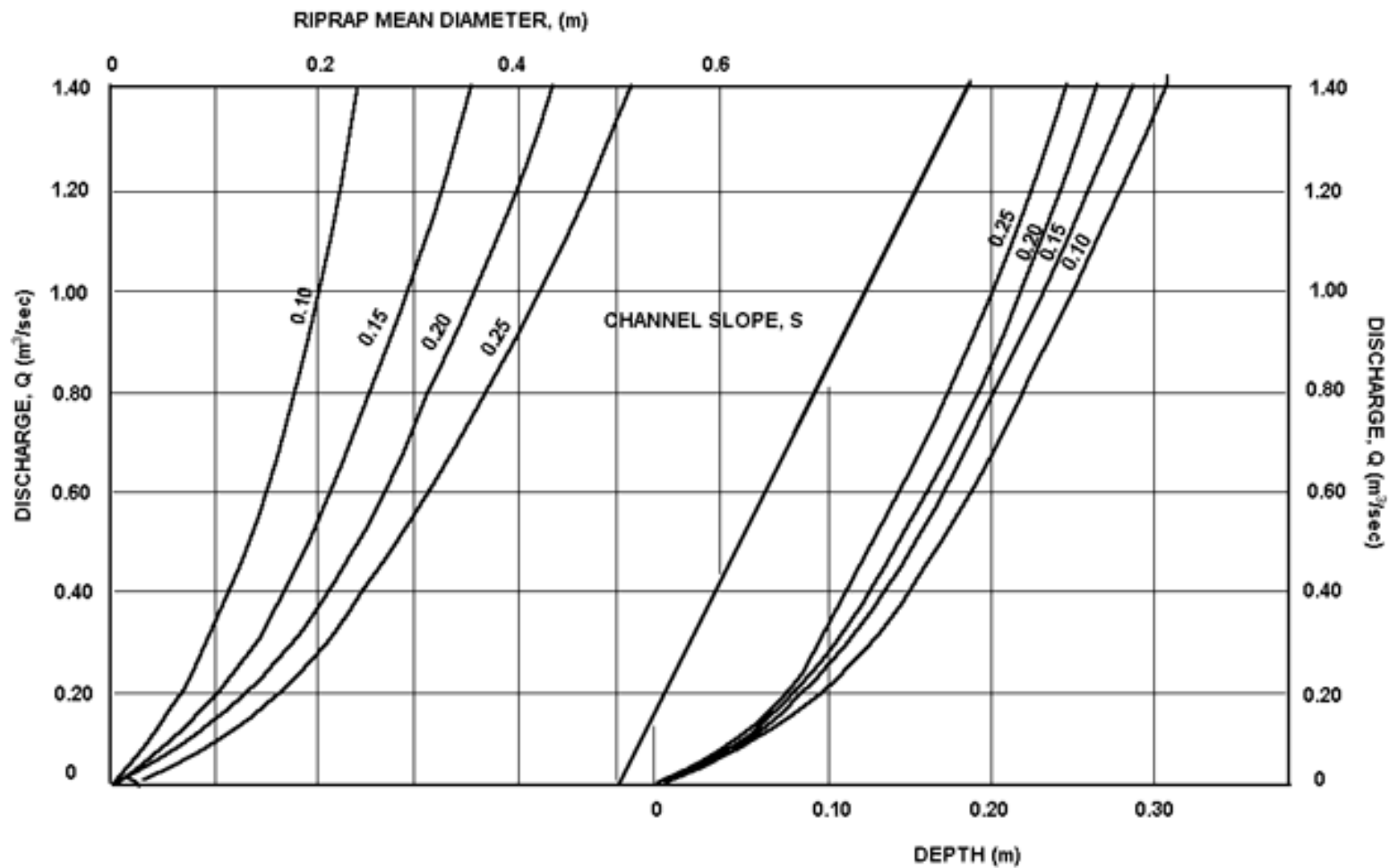
Chart 17. Steep Slope Riprap Design, B=1.2m, Z=3
