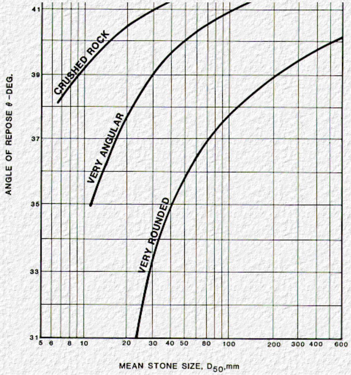
Chart 12. Angle of Repose Riprap in Terms of Mean Size and Shape of Stone
