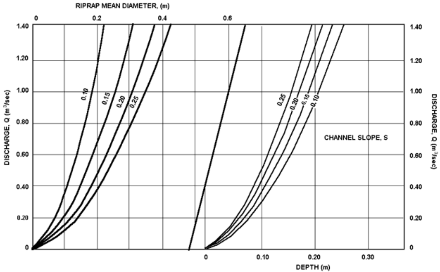
Chart 18. Steep Slope Riprap Design, B=1.8m, Z=3
