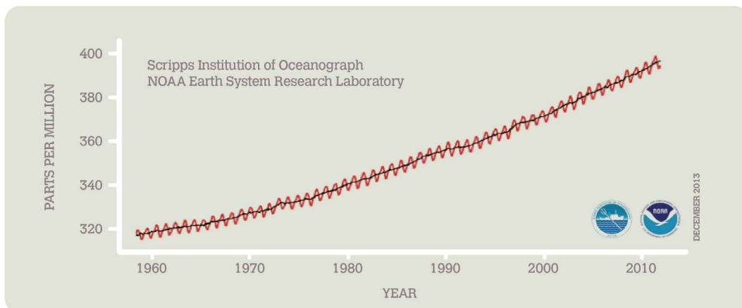
Graph: Atmospheric CO 2 at Mauna Loa Observatory, Hawaii
