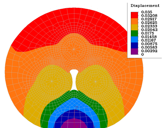
Figure 11 Displacement of Model
