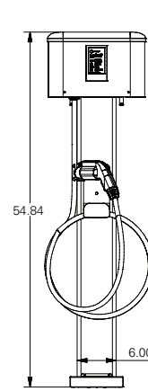
Dimensions (Shown with Advanced Cord Management)
