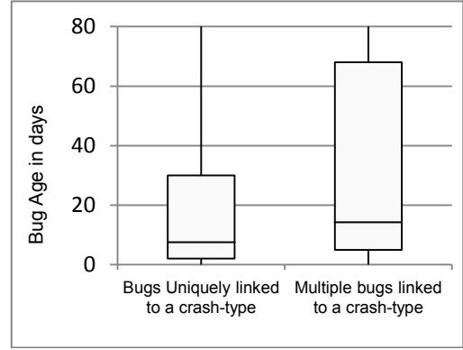
Figure 6: Boxplots comparing lifetimes of bugs uniquely linked to a crash-type vs bugs collectively linked to a crash-type
