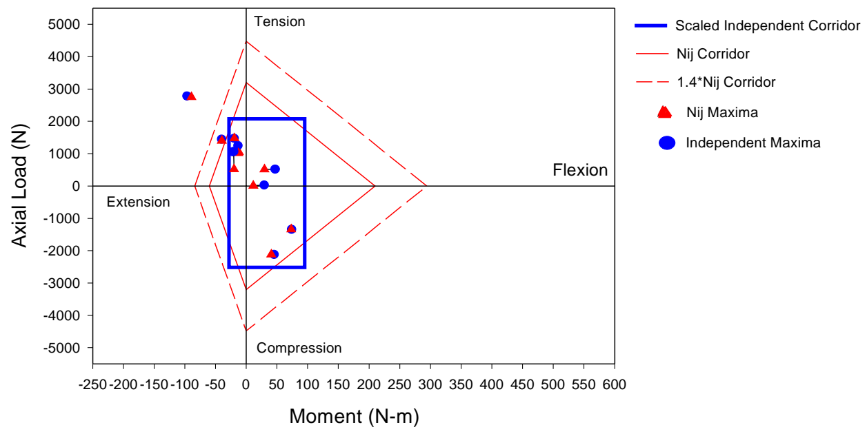
Figure A-9. Comparison of Neck Injury Criteria for Transport Canada Rigid Barrier Tests for 1998 Vehicles with 5% Female Dummy in the Passenger Position.
