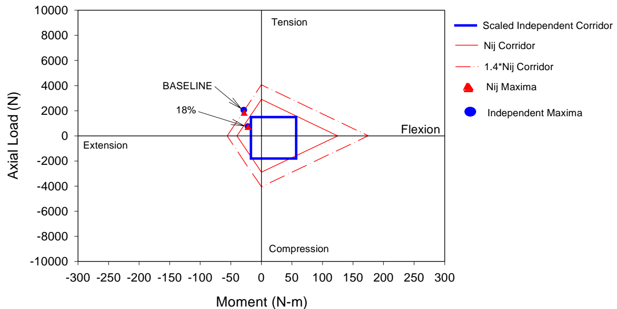
Figure A-19. Comparison of Neck Injury Criteria for Out-of-Position Tests with Hybrid III 6YO Dummy in ISO 1 Position using air bag system D, model year 1996. The labels indicate tests performed with the unmodified baseline system or with the inflator with 18 percent propellant removed.
