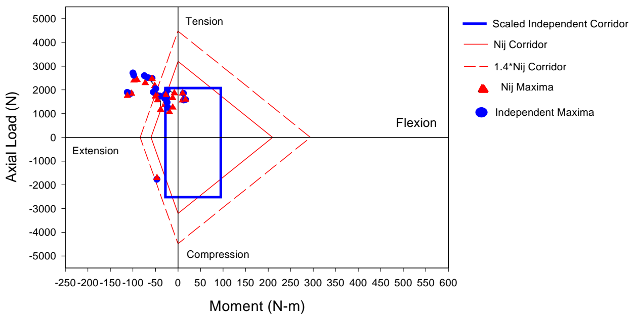
Figure A-8. Comparison of Neck Injury Criteria for Transport Canada Rigid Barrier Tests for pre-1998 Vehicles with 5% Female Dummy in the Driver Position.
