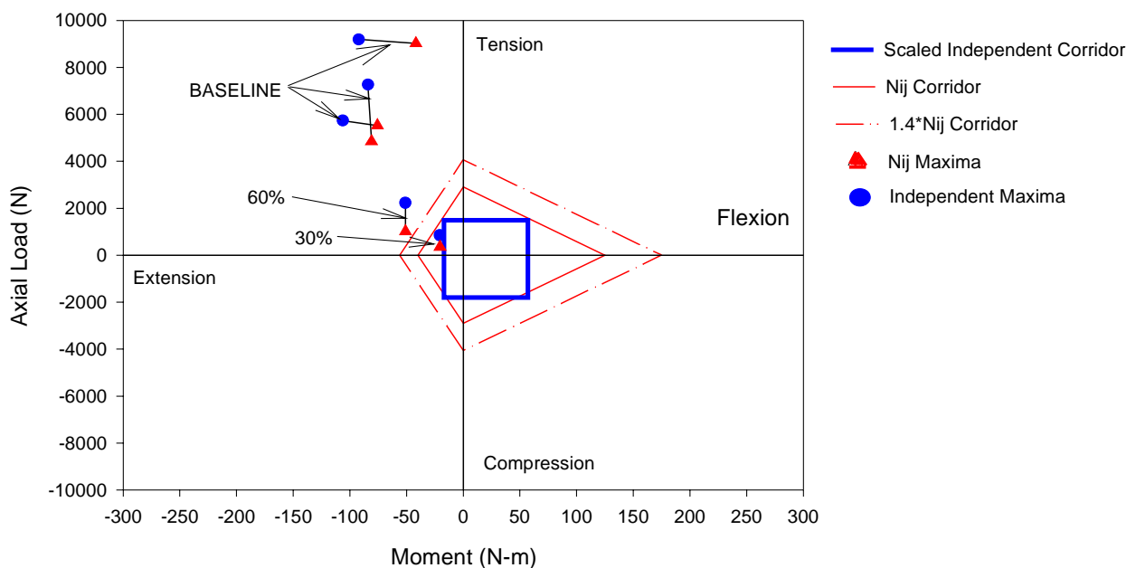
Figure A-18. Comparison of Neck Injury Criteria for Out-of-Position Tests with Hybrid III 6YO Dummy in ISO 2 Position using air bag system B, model year 1994. The labels indicate tests performed with the unmodified baseline system or with the inflator with 30 or 60 percent propellant removed.
