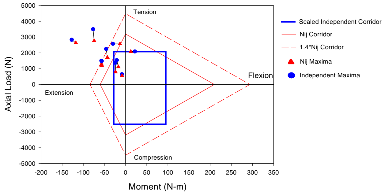
Figure A-11. Comparison of Neck Injury Criteria for Transport Canada Offset Frontal Tests for 1998 Vehicles with 5% Female Dummy in the Driver Position.
