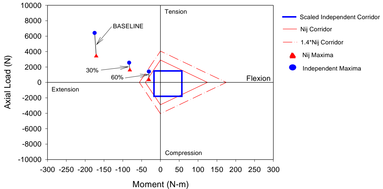
Figure A-17. Comparison of Neck Injury Criteria for Out-of-Position Tests with Hybrid III 6YO Dummy in ISO 1 Position using air bag system B, model year 1994. The labels indicate tests performed with the unmodified baseline system or with the inflator with 30 or 60 percent propellant removed.
