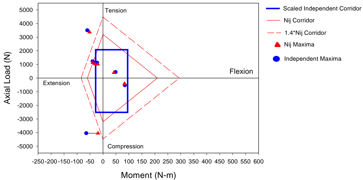
Figure A-14. Comparison of Neck Injury Criteria for Transport Canada Offset Frontal Tests for pre-1998 Vehicles with 5% Female Dummy in Passenger Position.
