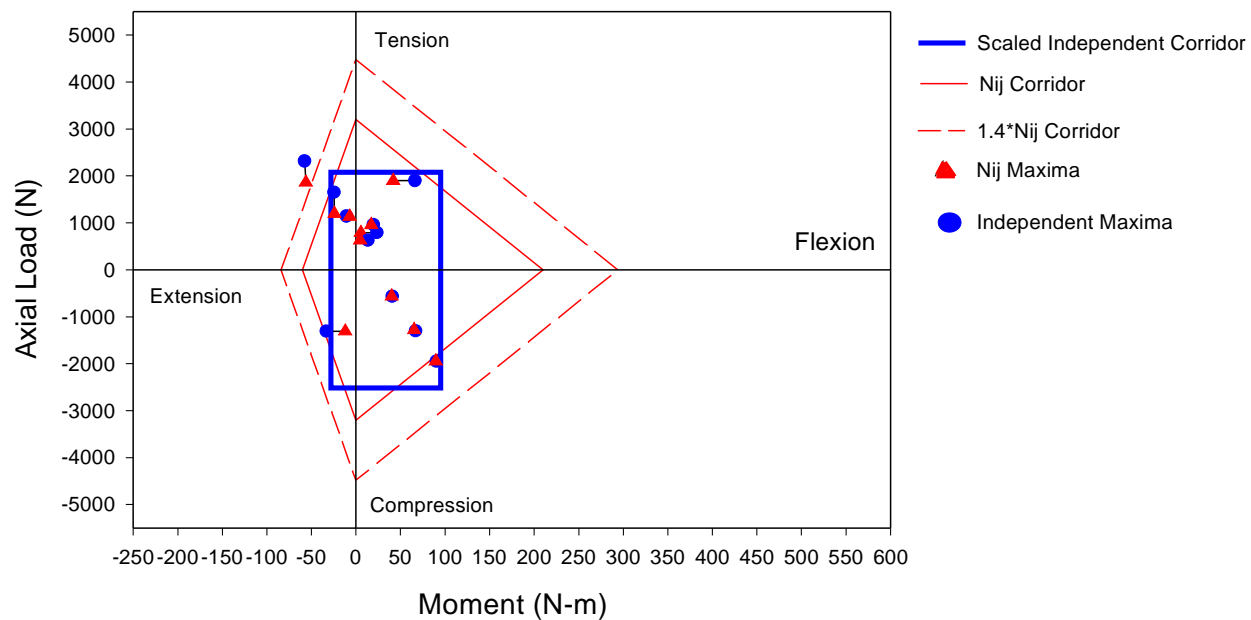
Figure A-13. Comparison of Neck Injury Criteria for Transport Canada Offset Frontal Tests for 1998 Vehicles with 5% Female Dummy in the Passenger Position.
