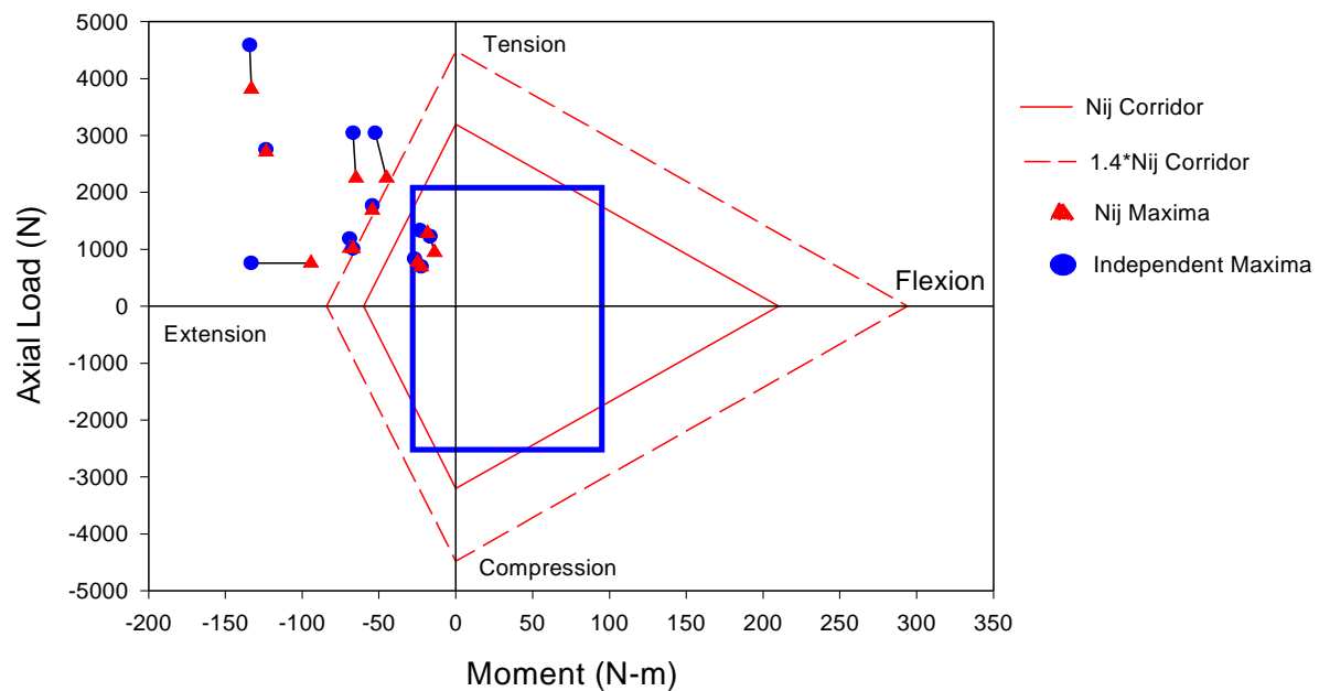
Figure A-12. Comparison of Neck Injury Criteria for Transport Canada Offset Frontal Tests for pre-1998 Vehicles with 5% Female Dummy in the Driver Position.
