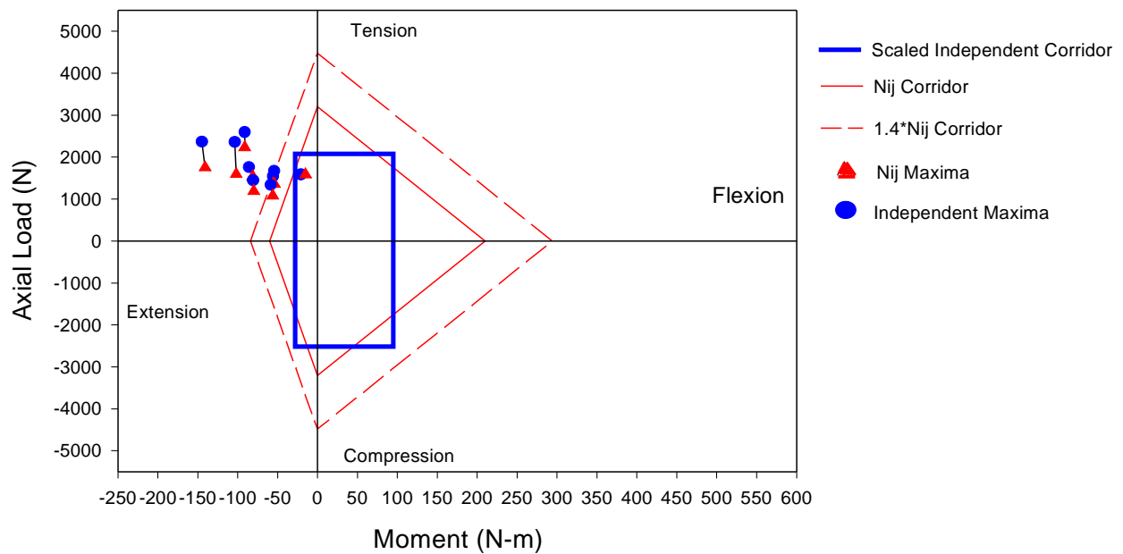
Figure A-15. Comparison of Neck Injury Criteria for Out-of-Position Tests with Hybrid III 5% Female in ISO 1 Position.
