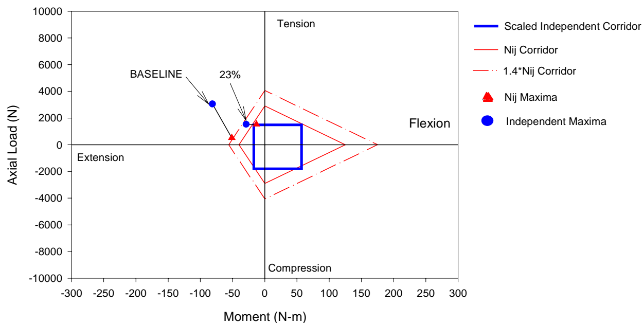
Figure A-22. Comparison of Neck Injury Criteria for Out-of-Position Tests with Hybrid III 6YO Dummy in ISO 2 Position using air bag system I, model year 1996. The labels indicate tests performed with the unmodified baseline system or with the inflator with 23 percent propellant removed.
