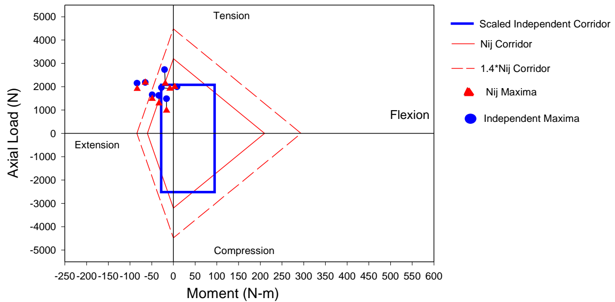
Figure A-7. Comparison of Neck Injury Criteria for Transport Canada Rigid Barrier Tests for 1998 Vehicles with 5% Female Dummy in the Driver Position.
