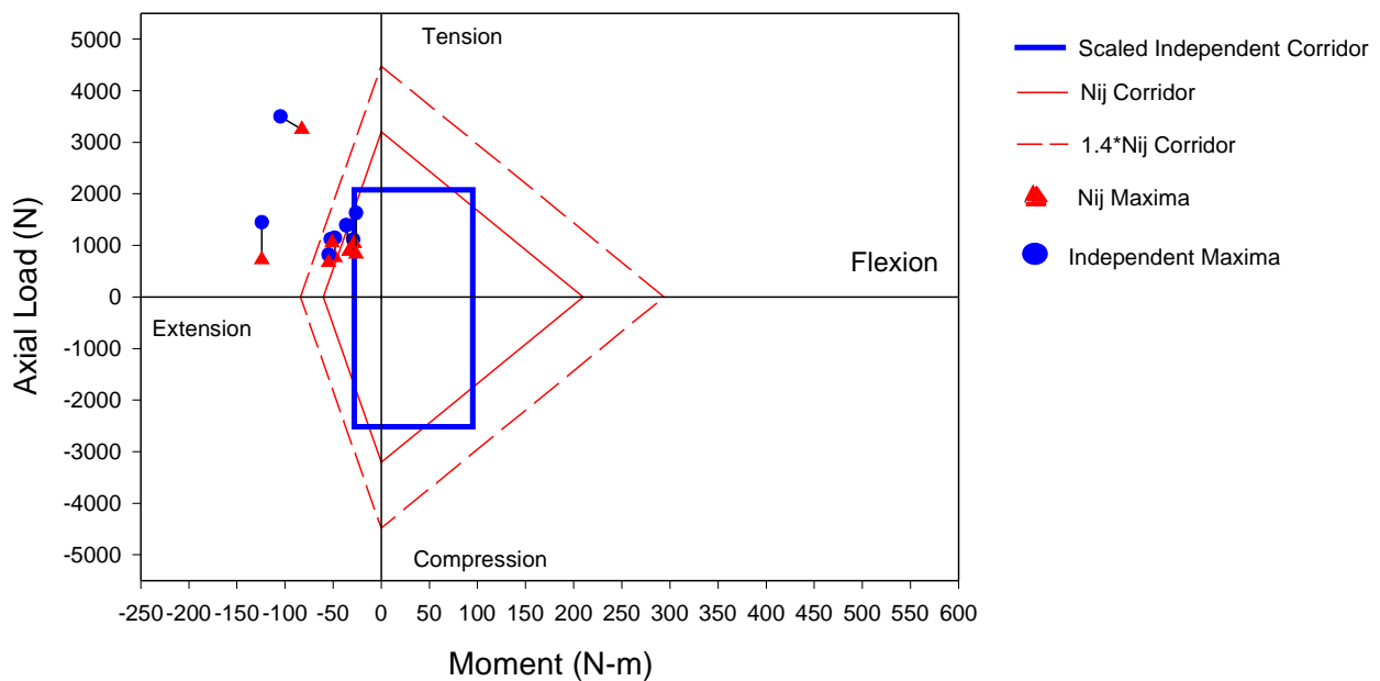
Figure A-16. Comparison of Neck Injury Criteria for Out-of-Position Tests with Hybrid III 5% Female in ISO 2 Position.
