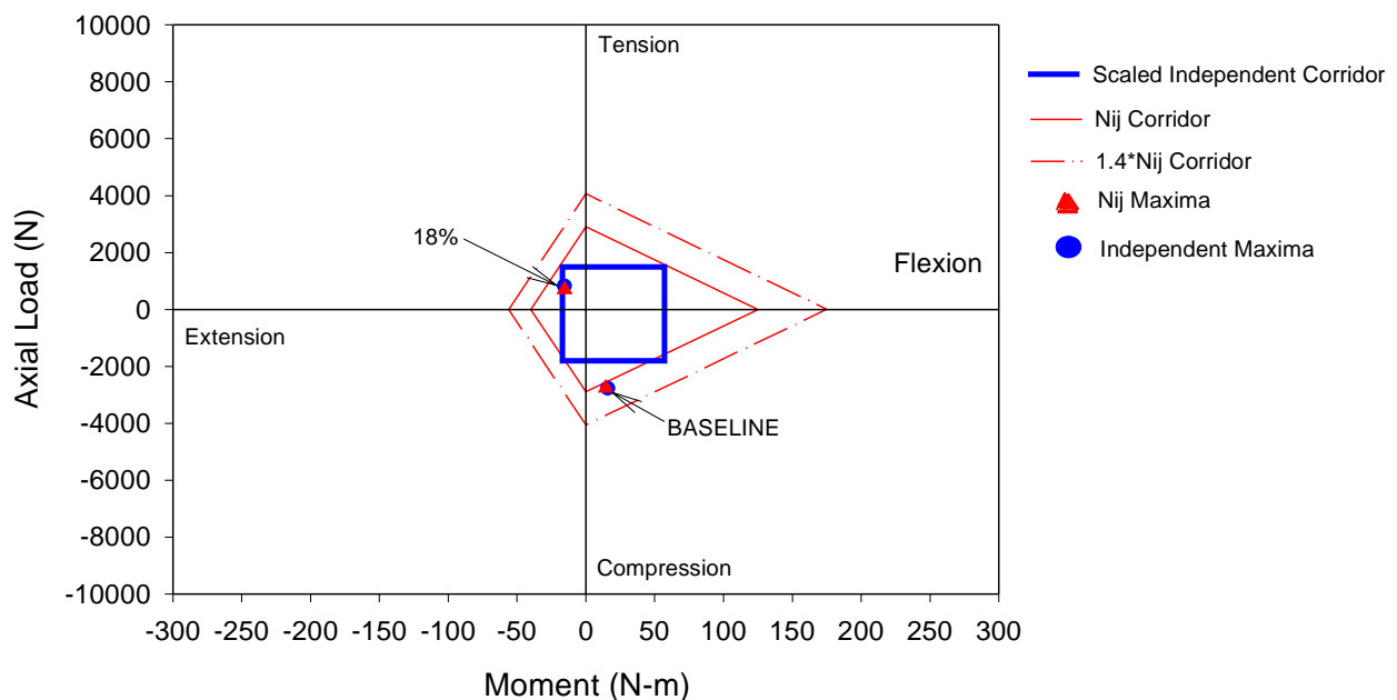
Figure A-20. Comparison of Neck Injury Criteria for Out-of-Position Tests with Hybrid III 6YO Dummy in ISO 2 Position using air bag system D, model year 1996. The labels indicate tests performed with the unmodified baseline system or with the inflator with 18 percent propellant removed.
