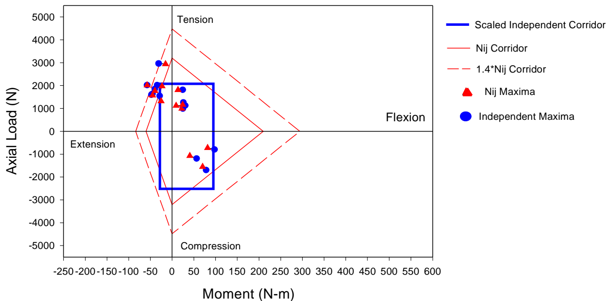
Figure A-10. Comparison of Neck Injury Criteria for Transport Canada Rigid Barrier Tests for pre-1998 Vehicles with 5% Female Dummy in Passenger Position.
