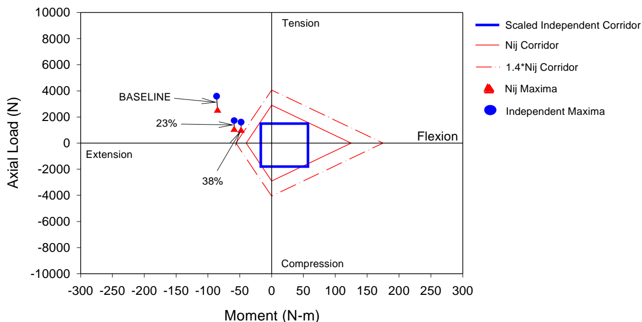
Figure A-21. Comparison of Neck Injury Criteria for Out-of-Position Tests with Hybrid III 6YO Dummy in ISO 1 Position using air bag system I, model year 1996. The labels indicate tests performed with the unmodified baseline system or with the inflator with 23 percent propellant removed
