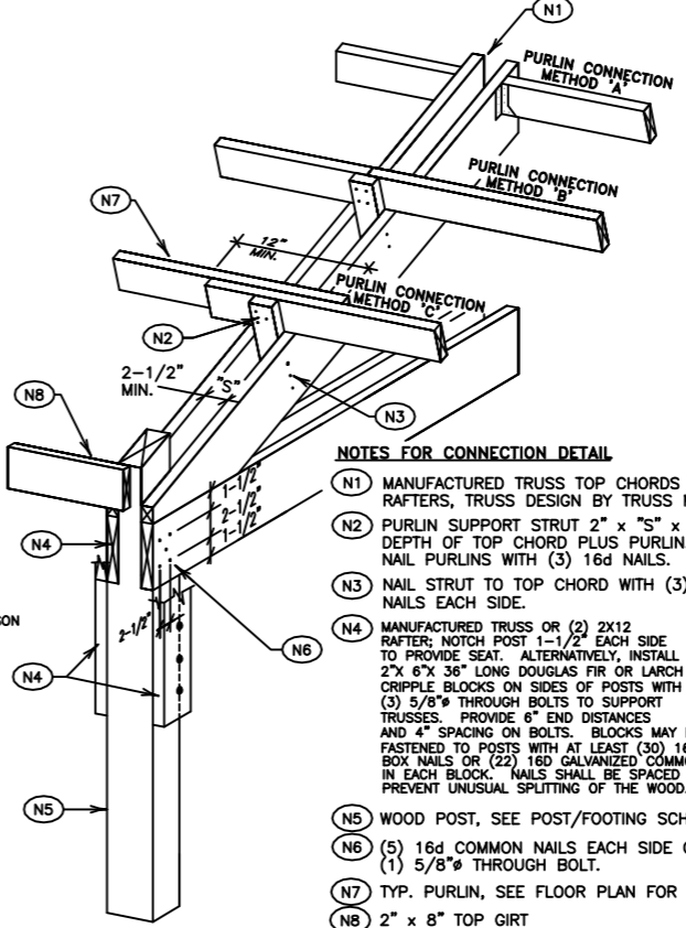
DETAIL 1 - TRUSS-COLUMN OR RAFTER-IN CONNECTION, PURLIN SUPPORT
