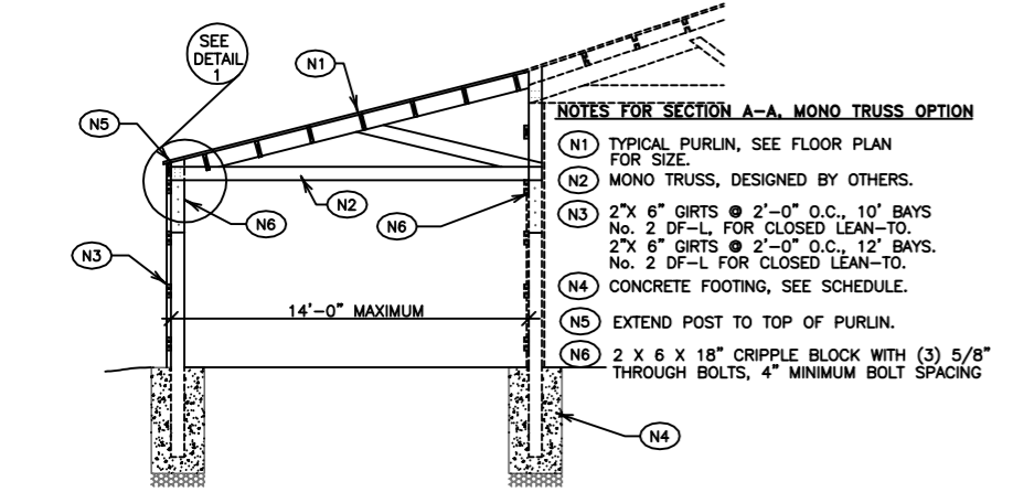
BUILDING SECTION A - A, MONO-TRUSS OPTION
