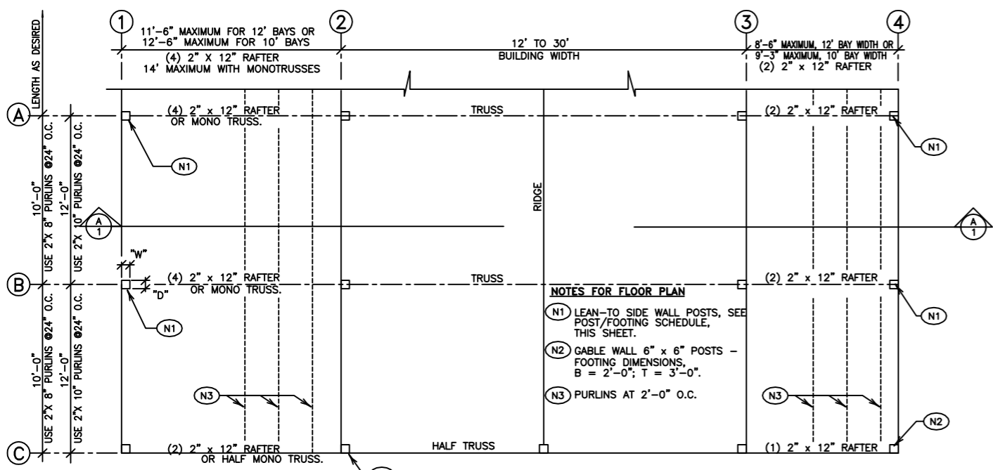
FLOOR PLAN
