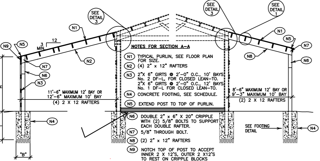
BUILDING SECTION A - A, RAFTER OPTION
