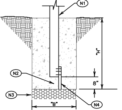
FOOTING DETAIL
