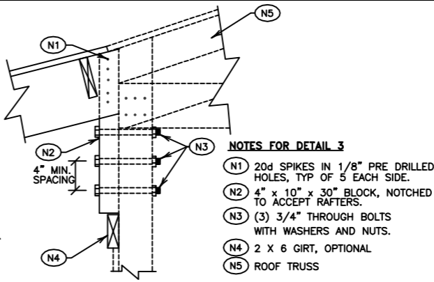
DETAIL 3 - OPTIONAL RAFTER COLUMN CONNECTION
