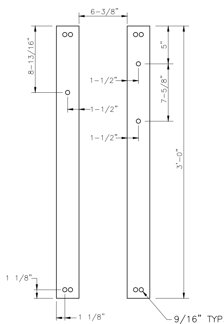
SIDE VIEW
