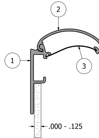
CROSS-SECTION OPEN
