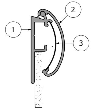
CROSS-SECTION CLOSED
