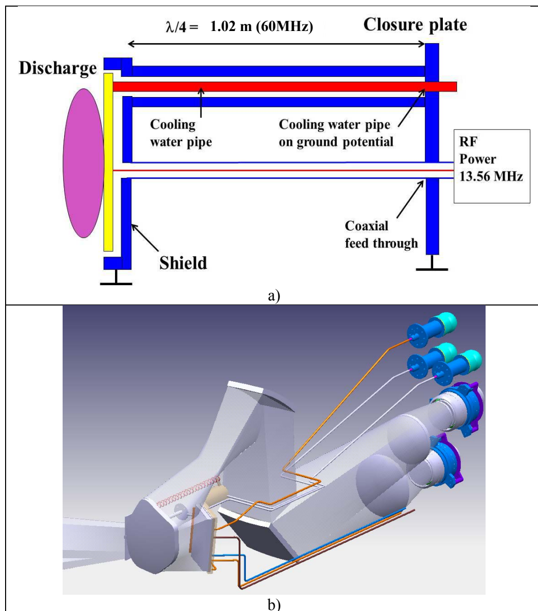
Fig. 4: Implementation concept for mirror cleaning showing a) schematic depiction of components of cleaning system, and b) rendering of MSE 1 st mirror in E3 equipped for cleaning with RF-produced argon plasma.
