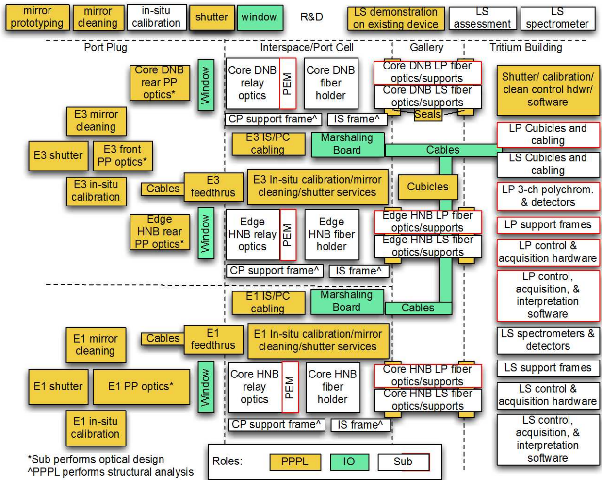
Figure 5 – Block diagram illustrating MSE design responsibilities (items with red outline will not be designed if there is a decision to implement only MSE-LS at HP1)
