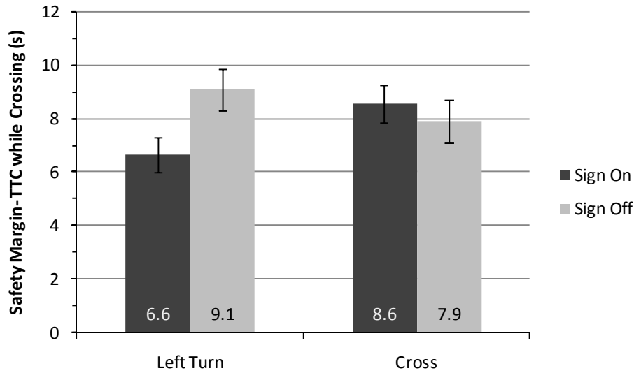
Figure 10. Safety margin for truck drivers while crossing from the stop sign for both left turn and crossing maneuvers.
