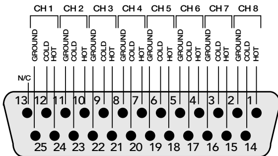
Analog DB25 Line-Level Input and Output
