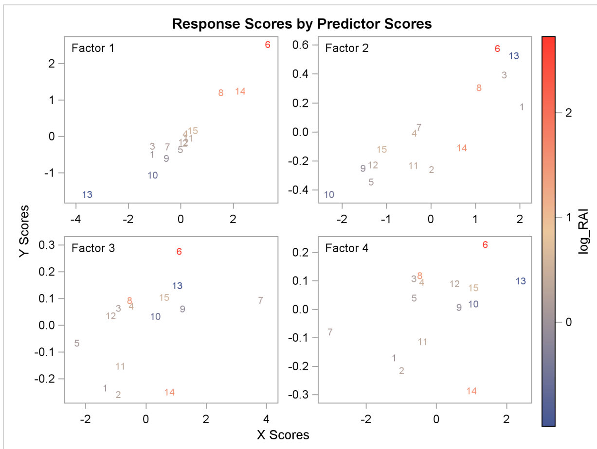
Output 67.1.4 X-Scores versus Y-Scores
