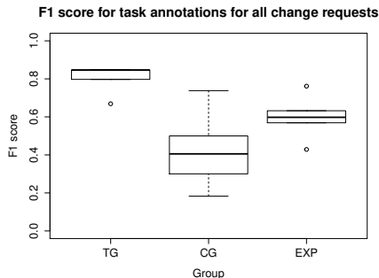
Figure 4: F1 score for task annotations for all change requests
