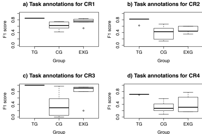
Figure 3: F1 score for task annotations for individual change requests
