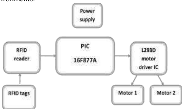
Figure 1. Schematic of the Project
