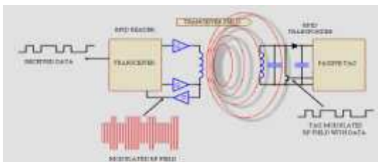
Figure 3. Typical RFID System
