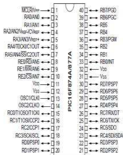
Figure 2. Pin Diagram of PIC16F877A
